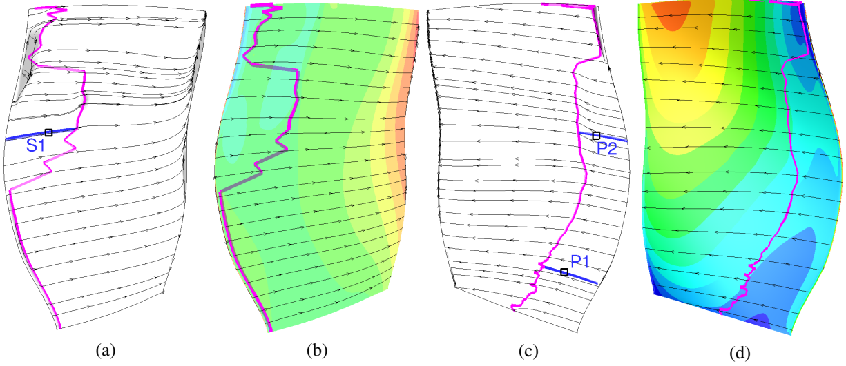
Fig. 5 (a) and (c): Friction lines at suction (a) and pressure (c) sides. The grey regions show where |\beta_0| > \pi/2 . (b) and (d): streamlines at suction (b) and pressure (d) sides and pressure contours. On all four figures, the thick pink line shows predicted transition locations in elsA.
