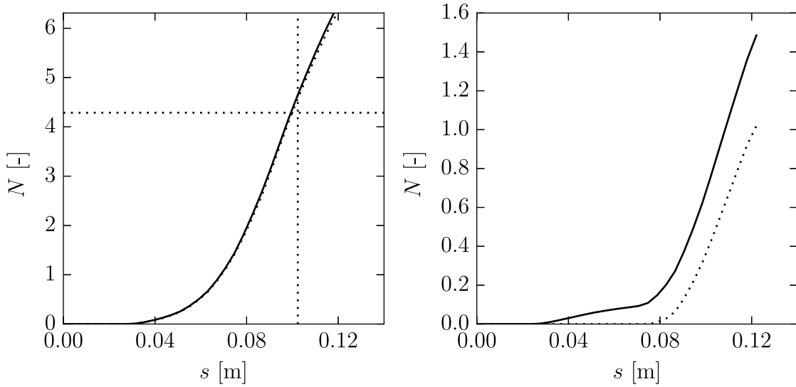
Fig. 9 N -factor against the curvilinear abscissa s along the line P2 for Tollmien-Schlichting (left) and stationary cross-flow (right) waves. See the legend figure 8.
