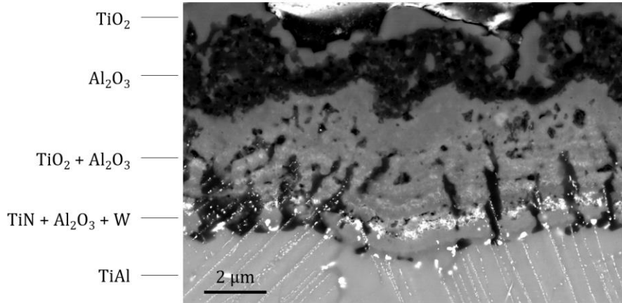
Figure 6: SEM-BSE image of the IRIS alloy after 1000 cycles in air at 800 °C.
