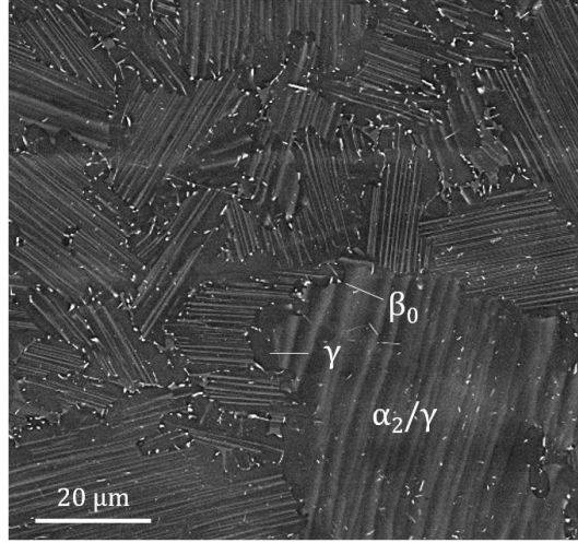
Figure 1: SEM micrograph of as-prepared IRIS alloy showing the lamellar \alpha_2/\gamma grains, with a \gamma band and \beta_0 precipitates at the grain boundaries.
