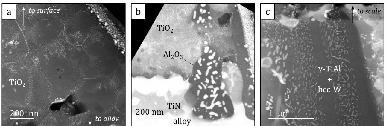
Figure 8: STEM-HAADF images of the reaction product formed on the IRIS alloy after 1000 cycles in air at 800 °C. (a) \text{TiO}_2 grains in the \text{TiO}_2 - \text{Al}_2\text{O}_3 layer with intergranular W-rich particles (see also supplementary material S1), (b) \text{Al}_2\text{O}_3 chimney across the \text{TiN}/\text{TiO}_2 interface with intragranular W-rich particles, (c) alloy near the alloy/scale interface, showing that the \alpha_2 lamellae have been destabilized and converted to fine bcc-W particles.
