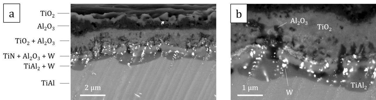
Figure 4: SEM micrograph in backscattered electron mode (BSE) of the IRIS alloy after 100 h oxidation in air at 800 °C. (a) Overview of the oxidation products; (b) detailed view of the alloy/scale interface.
