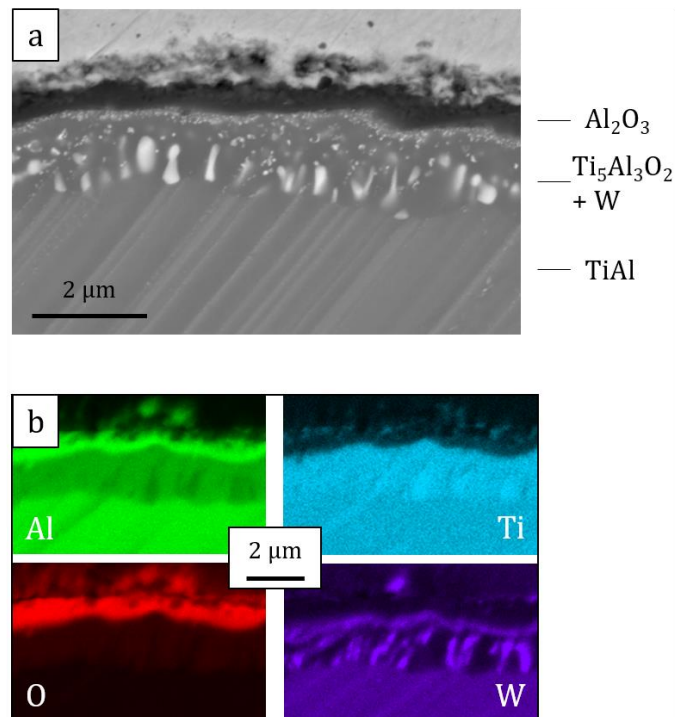
Figure 9: SEM analysis of the IRIS alloy after 100 h oxidation in Ar-21O 2 at 800 °C. (a) BSE view; (b) X-ray maps.
