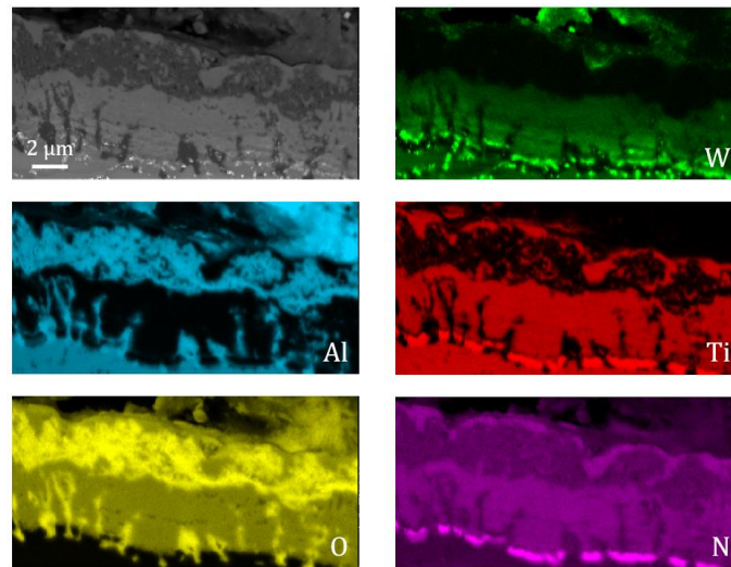
Figure 7: SEM-BSE image and X-ray maps of the reaction product on the IRIS alloy after 1000 cycles in air at 800 °C.
