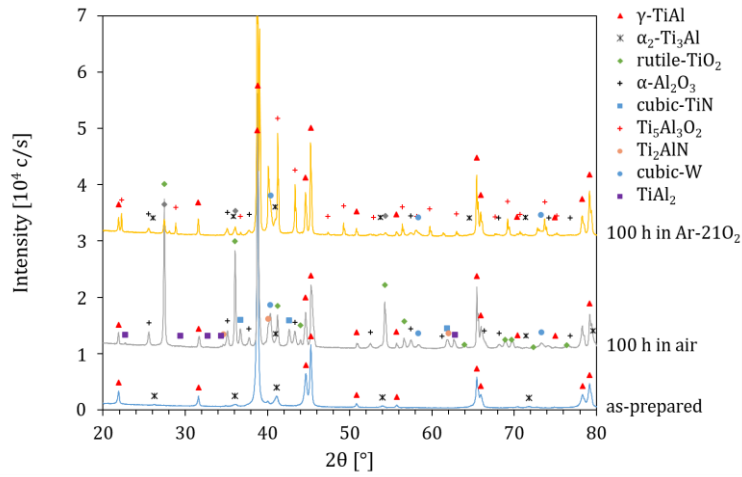
Figure 2: XRD patterns measured on the IRIS alloy in the as-prepared state and after 100 h oxidation in air and in Ar-21O 2 at 800 °C.
