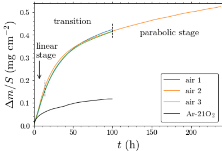
Figure 3: Thermogravimetric analysis of the IRIS alloy at 800°C in air and Ar-21O 2 .
