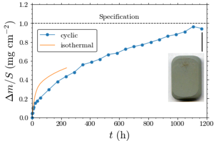
Figure 5: Mass gains of the IRIS alloy during cyclic oxidation in laboratory air at 800 °C. The insert shows a photograph of the specimen at the end of the 1000 cycles. The mass gains measured in the 240 h isothermal TGA test are included for comparison.
