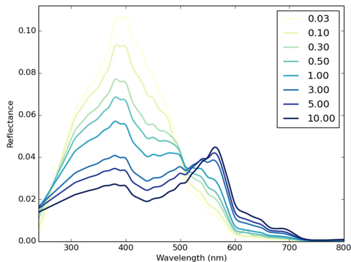
Figure 2. Ocean column reflectance for eight values of the chlorophyll concentration (0.03, 0.1, 0.3, 0.5, 1, 3, 5, 10 \text{mg}\cdot\text{m}^{-3} ) used in the ADAM API toolkit derived from the COART model.
