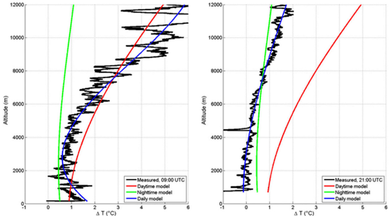
FIG. 5. Difference in temperature between the temperature close to the capacitive sensor and the air temperature sensor. The black line corresponds to the measured value, and the red, green, and blue lines correspond to the different models described in section 3c. Shown are radiosoundings launched at (left) the SIRTA observatory at 0900 UT 24 Aug 2018 and (right) the OHP at 2100 UT 21 Sep 2011.
