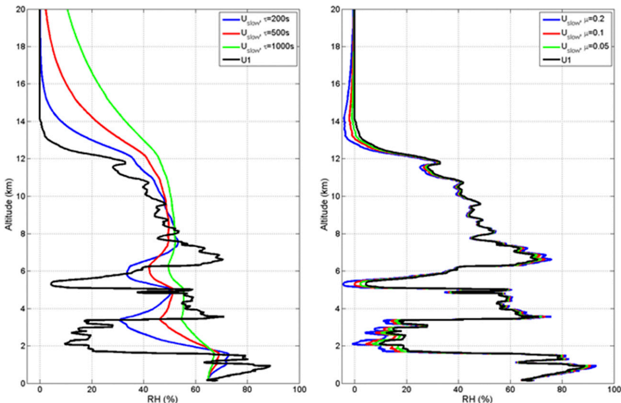
FIG. 4. Vertical profile of the raw relative humidity and relative humidity of the slow regime for (left) three time constants ( \tau = 200, 500, 1000 s), with a fixed ratio of the slow to fast response sensors \mu = 0.1 , and (right) three ratios of the slow to fast response sensors ( \mu = 0.2, 0.1, 0.05 ) with a fixed time constant \tau = 500 s at 0900 UT 24 Aug 2018 at the Sirta observatory.
