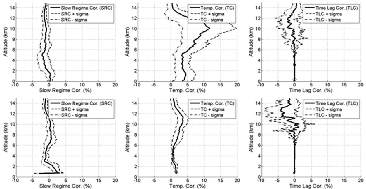
FIG. 7. Vertical profile of (left) the slow-regime correction, (center) the temperature correction, and (right) the time-lag correction for (top) the 25 radiosoundings launched at the Sirta observatory for the daytime period and (bottom) the 20 radiosoundings launched at the OHP Observatory for the nighttime period. The average value is plotted as a thick line, and the standard deviation is shown with dashed lines.
