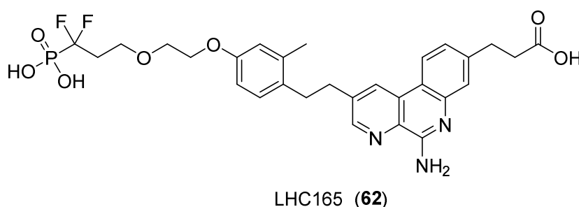
Figure 31 : A TLR7 agonist belonging to Novartis pipeline
