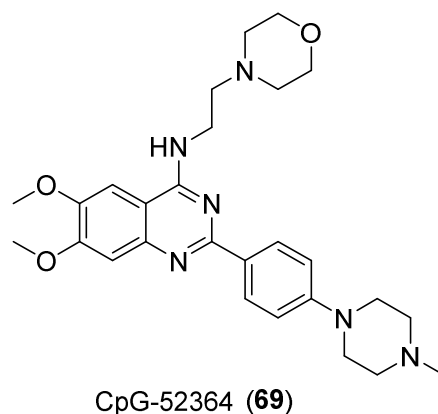
Figure 36 : Quinazoline derivative
