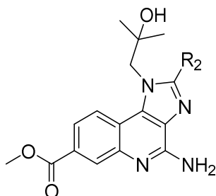
Figure 26 : Core-structure of the imidazo[4,5- c ]quinoline series [249]
