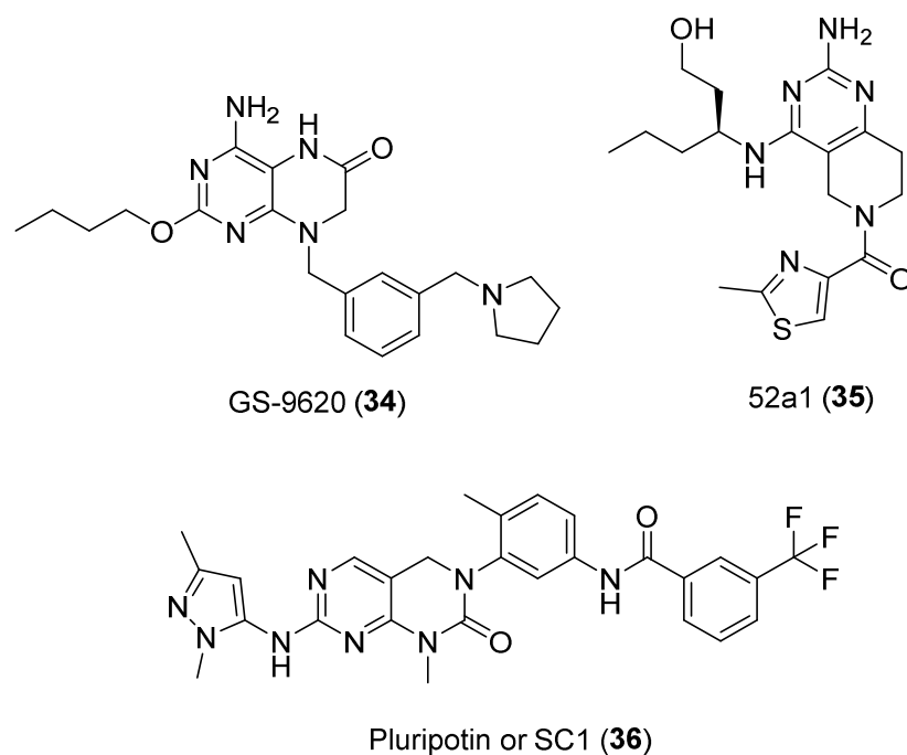
Figure 18 : Annulated pyrimidine derivatives
