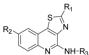
Core-structure of the thiazolo[4,5-c]quinoline series
