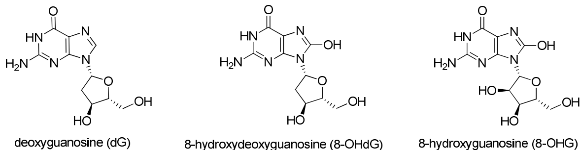
Figure 4 : Guanosine derivatives
