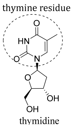
Figure 32 : Thymidine nucleoside
