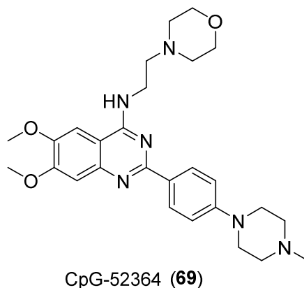
Figure 36 : Quinazoline derivative
