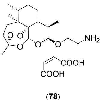
Figure 41 : Artemisinin analogue
