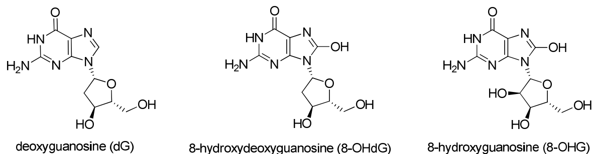
Figure 4 : Guanosine derivatives
