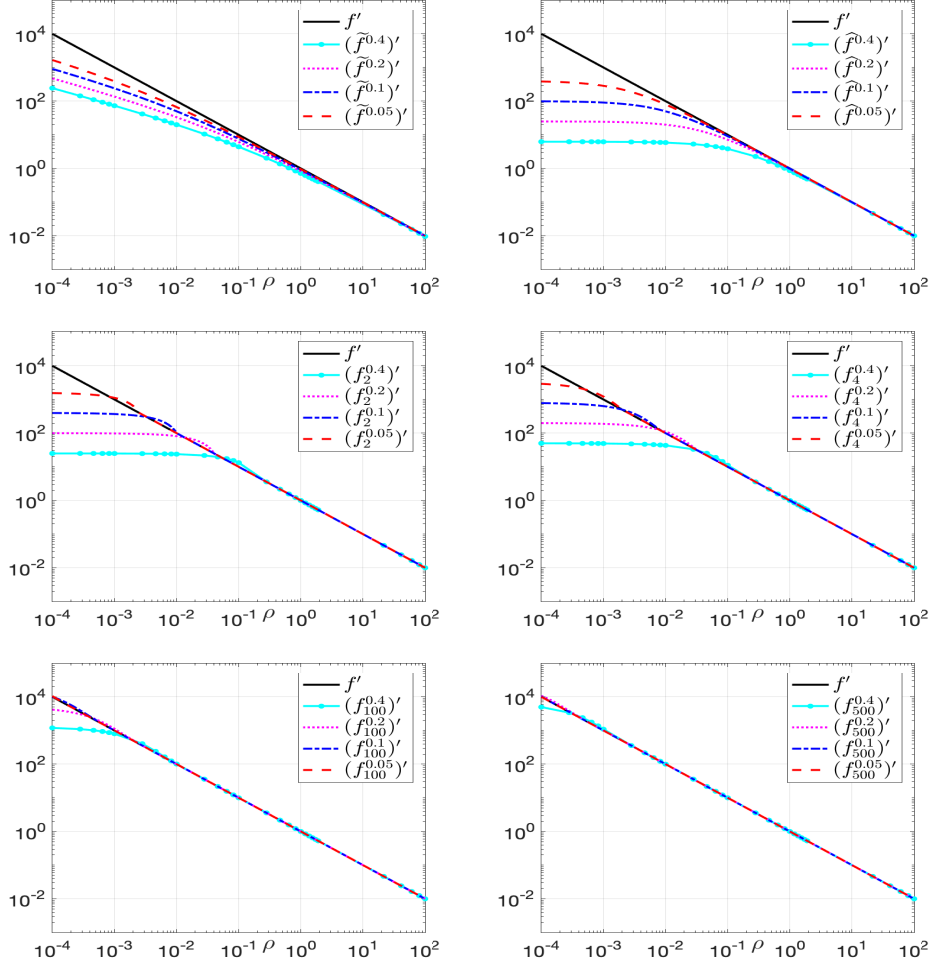
FIGURE 3. Comparison of different regularizations for f'(\rho) = 1/\rho .
