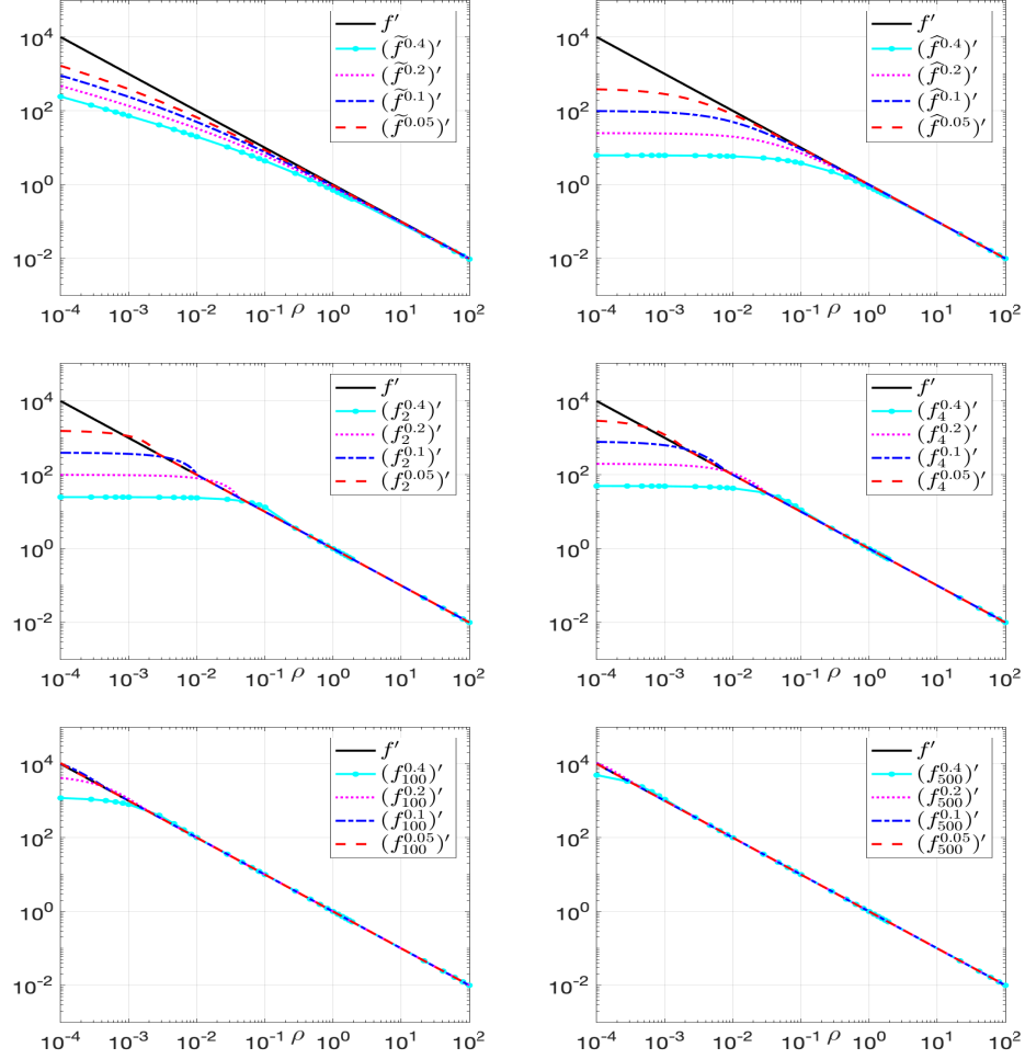
FIGURE 3. Comparison of different regularizations for f'(\rho) = 1/\rho .
