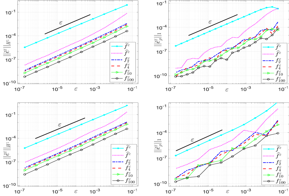
FIGURE 6. Convergence of the RLogSE (5.1) with various regularized nonlinearities f_{\text{reg}}^\varepsilon to the LogSE (1.1), i.e., the error \|e^\varepsilon(t)\|_{H^1} and \|\check{e}_\rho^\varepsilon(t)\|_1 versus the regularization parameter \varepsilon at t = 3 for d = 1 (upper) and t = 2 for d = 2 (lower).
