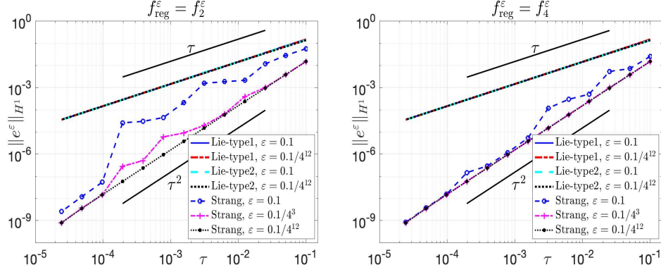
FIGURE 8. Convergence of the type-1 LTSP (4.7) & type-2 LTSP (4.20) as well as the STSP (4.33) to the ERLogSE (3.2) with regularized nonlinearity f_2^\epsilon (left) and f_4^\epsilon (right), i.e., errors \|e^\epsilon(3)\|_{H^1} versus \tau for various \epsilon .
