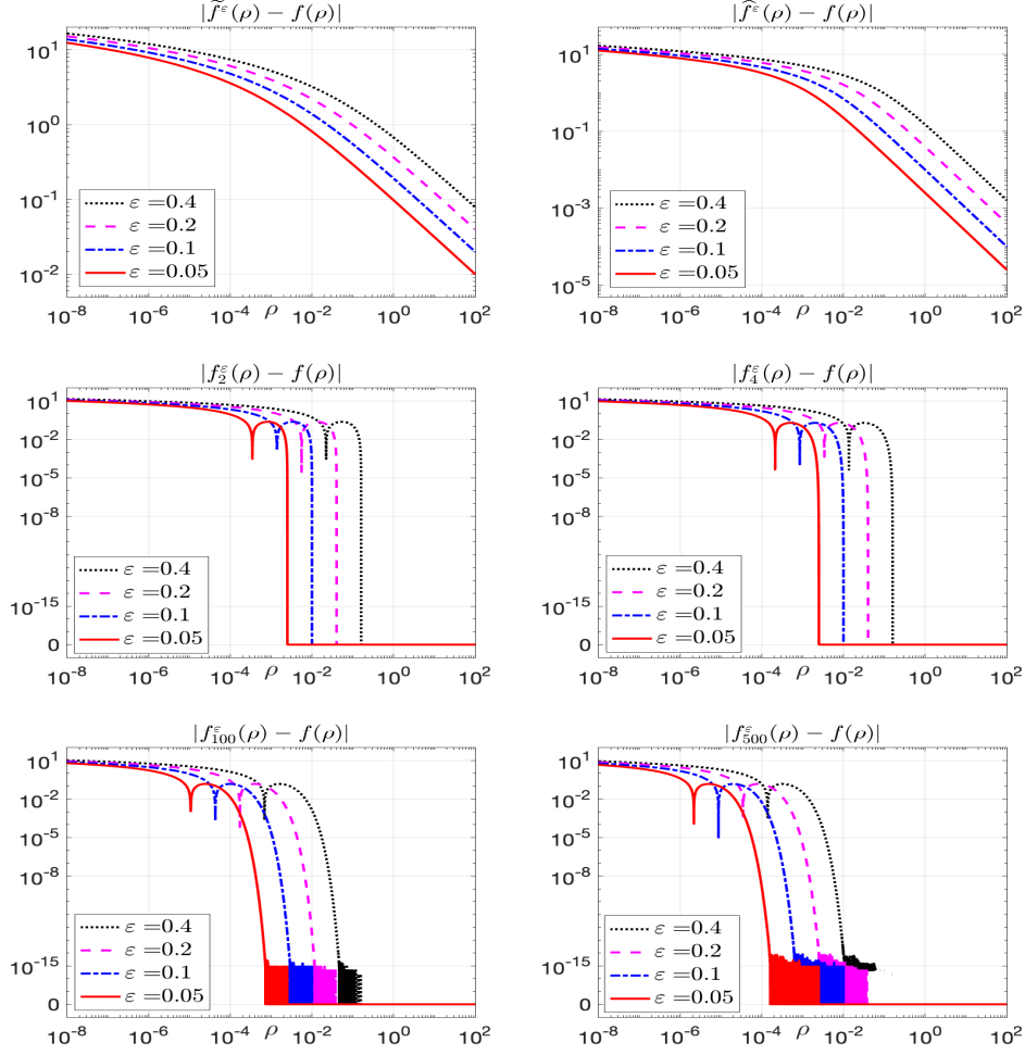
FIGURE 2. Comparison of different regularizations for the nonlinearity f(\rho) = \ln \rho .
