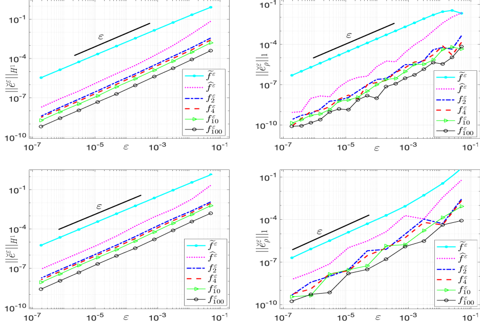
FIGURE 6. Convergence of the RLogSE (5.1) with various regularized nonlinearities f_{\text{reg}}^\varepsilon to the LogSE (1.1), i.e., the error \|\check{e}^\varepsilon(t)\|_{H^1} and \|\check{e}_\rho^\varepsilon(t)\|_1 versus the regularization parameter \varepsilon at t = 3 for d = 1 (upper) and t = 2 for d = 2 (lower).
