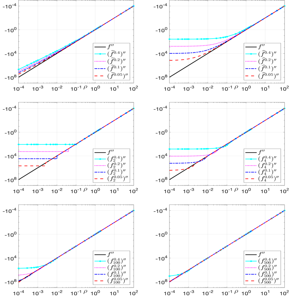
FIGURE 4. Comparison of different regularizations for f''(\rho) = -1/\rho^2 .
