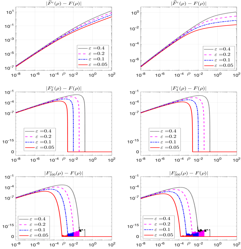
FIGURE 1. Comparison of different regularizations for F(\rho) = \rho \ln \rho - \rho .
