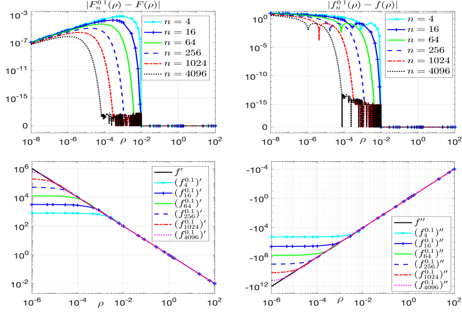
FIGURE 5. Comparison of regularizations g_n^{0.1} ( g = F, f, f', f'' ) with different order n .
