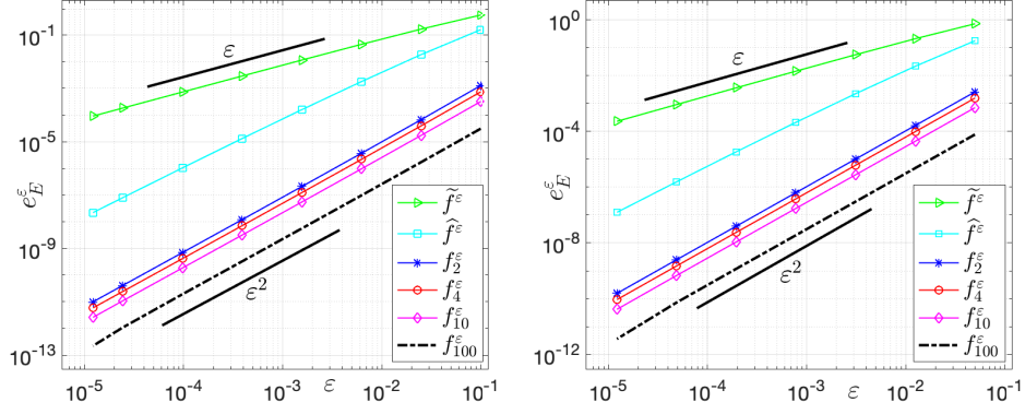
FIGURE 7. Convergence of the RLogSE (5.1) with various regularized nonlinearities f_{\text{reg}}^\epsilon to the LogSE (1.1): the energy error e_E^\epsilon(t) (5.4) at t = 3 for d = 1 (left) and t = 2 for d = 2 (right).
