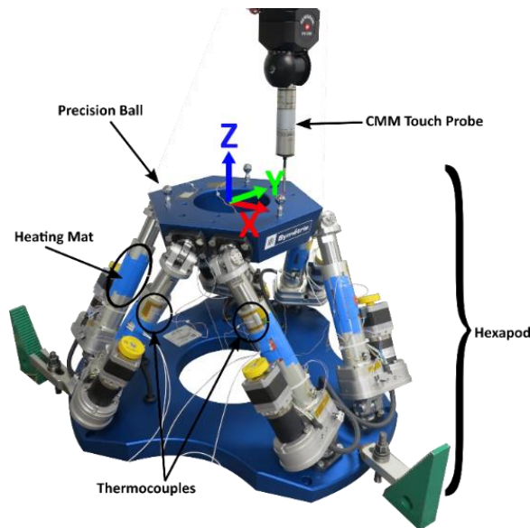
Figure 4. Test setup
