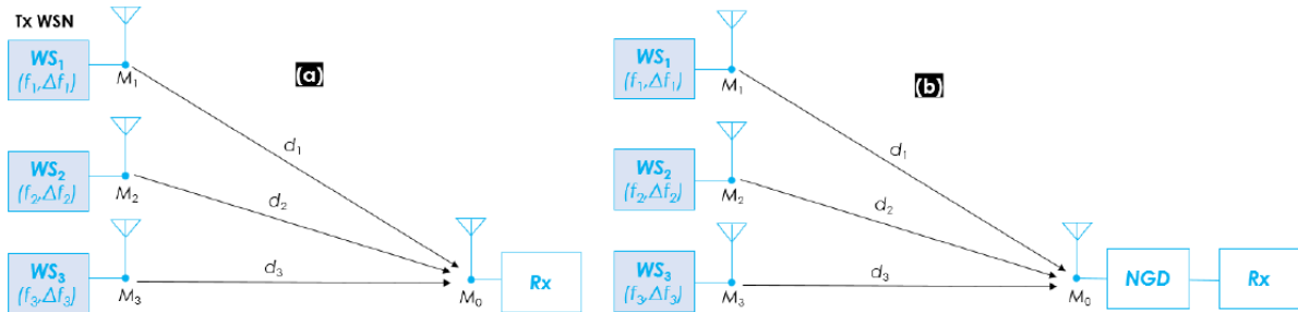
Figure 5: Configuration NGD delay reduction [7]
