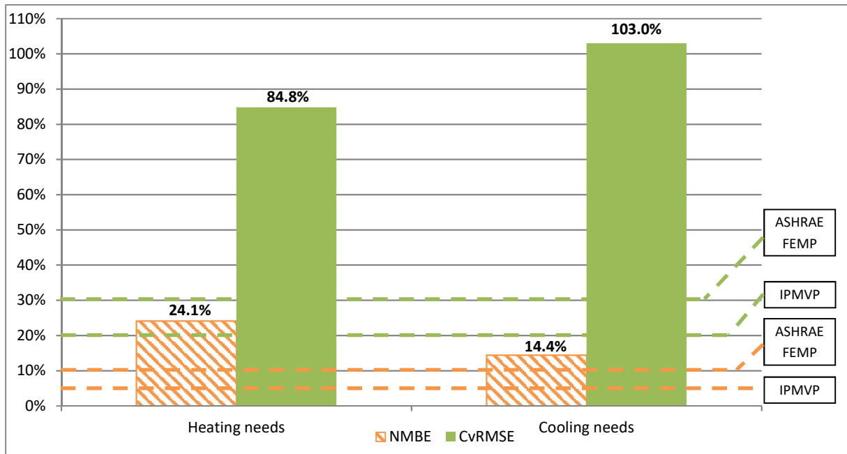
Figure 9: Calibration performance indicators in heating and cooling mode and guidelines thresholds for an hourly calibration
