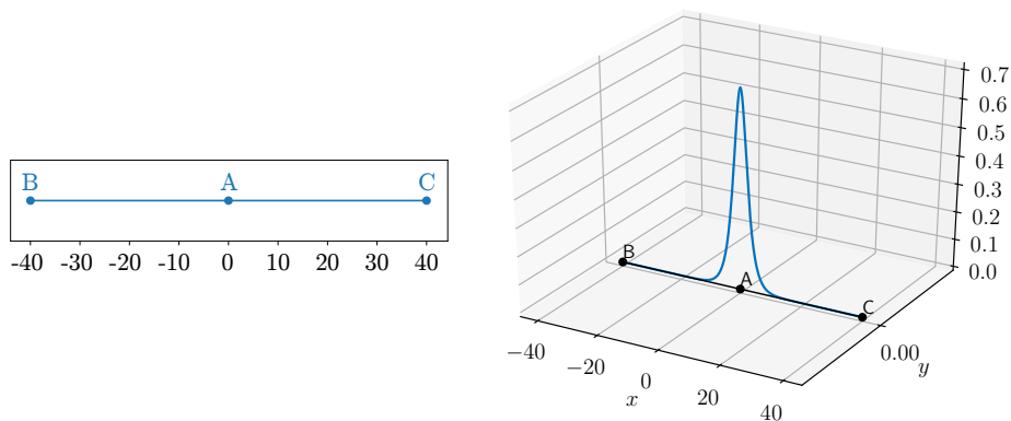
FIGURE 9. Two-edges graph (left) and the exact solution \phi_m(x) for m = 2 (right)
