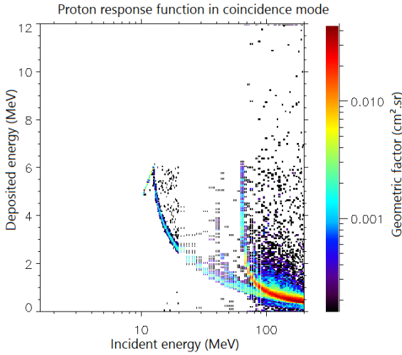
Fig. 4. Proton response function in coincidence mode. Geometric factor ( \text{cm}^2.\text{sr} ) in incident energy (x-axis)-deposited energy (y-axis) map.
