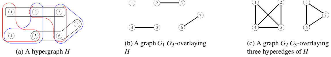
FIGURE 1: An example of two problems on hypergraph H . In the figure 1b, each hypergraph (e.g. S_1 = \{1,4,5\} ) is overlaid by a graph with three vertices and one edge (e.g. the edge in G[S_1] is (4,5) ). In the figure 1c, G_2 overlays three hyperedges S_1, S_2 = \{2,4,5\}, S_3 = \{3,6,7\} , each induced subgraph G[S_i] (for i = \{1,2,3\} ) is a C_3 graph.
