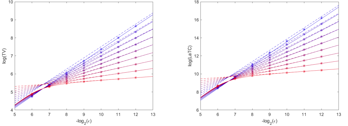
FIGURE 12. Log-log plots of TV and LTaC for fractional correlated standard Gaussian fields of size 2^{12} \times 2^{12} pixels for \alpha varying between 0.1 (in blue) and 0.9 (in red), as functions of the resolution \varepsilon . Empirical values are plotted with stars and theoretical ones are plotted with dashed curves for \varepsilon^{2\alpha} \lambda_{2\alpha} and with continuous curves for \beta_0(\varepsilon) .
