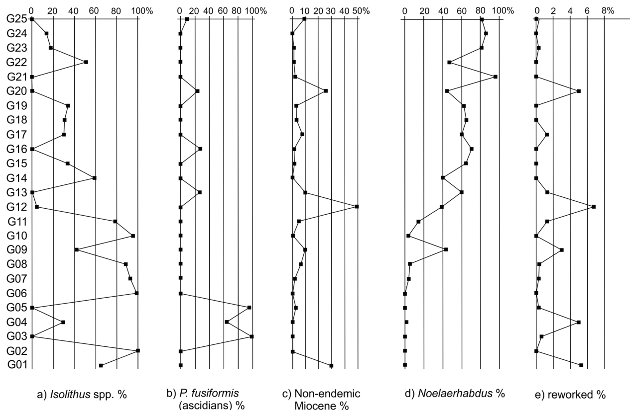
Figure 7: Distribution and ratio of calcareous nannoplankton taxa within the Guşteriţa 4 section. Numbers indicate the sampling levels (G01 to G25).
