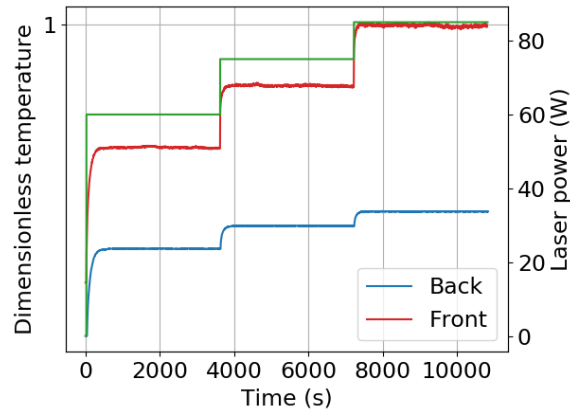
FIGURE 2: Laser power in green, dimensionless temperature profiles measured by the infrared camera in red and by the pyrometer in blue during the test
