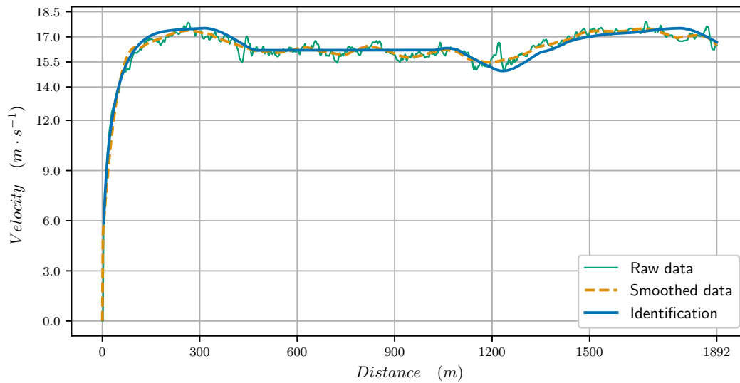
Fig 5. Velocity data (raw and smoothed, t_f = 116.460\text{s} ) and computed velocity ( t_f = 116.460\text{s} ) for the identified parameters for the 1900 meters race
