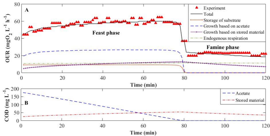
Fig. 8. Oxygen uptake rate (A) and substrate behaviour expressed as COD (B) for the individual processes during the acetate degradation for M1 theory (176 mgCOD L -1 ).
