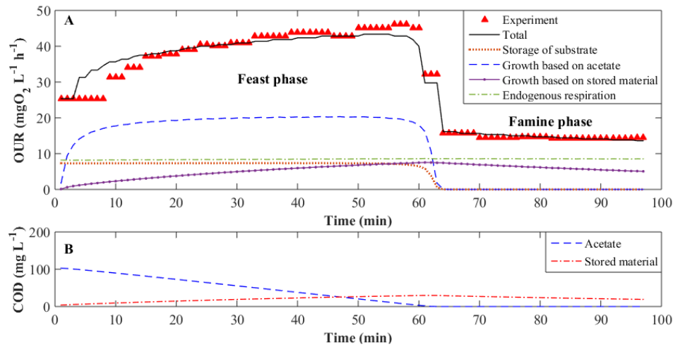
Fig. 7. Oxygen uptake rate (A) and substrate behaviour expressed as COD (B) for the individual processes during the acetate degradation for M1 theory (103 mgCOD L -1 ).
