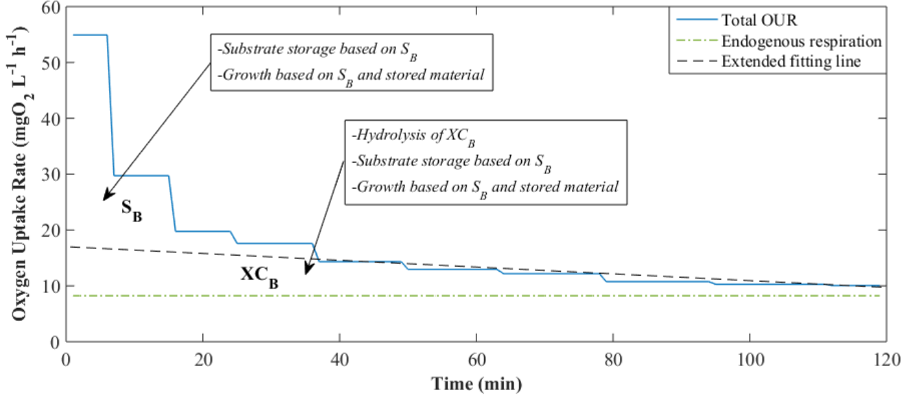
Fig. 4. Determination of the oxygen consumption for S_B and XC_B degradation taking into account simultaneous growth and substrate storage.
