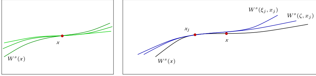
FIGURE 1. On the left, a generic point x with the local stable manifolds W_{\text{loc}}^s(\xi, x) with (\xi_i)_{i \geq 0} which varies (see Step 1). On the right, the choice of the sequence (\zeta, x_j) gives a family of local stable manifolds (see Step 2).
