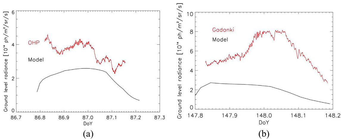
Fig. 7. (a) Comparisons between the measurement campaign at OHP, France in red and the model in black. (b) Same but for Gadanki, India. The model underestimates in both cases the intensity of the nightglow measured on the ground level, especially at Gadanki, where the night showed a strong activity of gravity waves.
