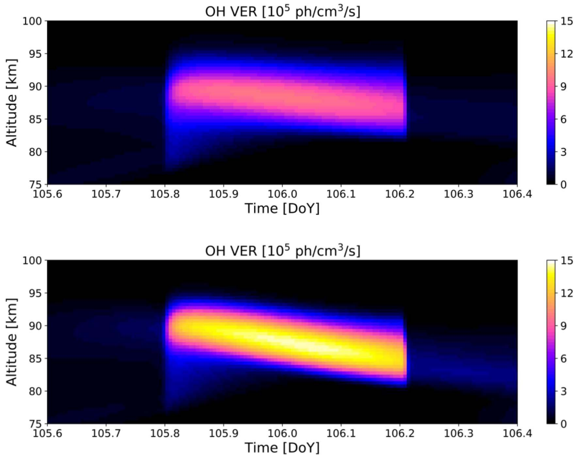
Fig. 4. Top panel: example of the OH volume emission rate (in 10^5 ph/cm 3 /s) between 80 km and 95 km for one night (starting at day of year [DoY] 105.8 and ending at DoY 106.2). Bottom panel: same example but with the tidal amplitude doubled.
