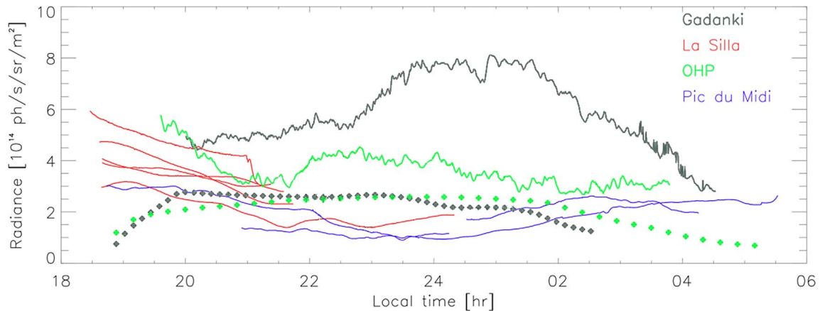
Fig. 8. Summary of the measurement campaigns (in solid lines) carried out by ONERA. Besides Gadanki and OHP (Fig. 7), campaigns have been performed at La Silla (Chile) and Pic du Midi (France). The crosses represent the evolution of the nightglow modeled at the ground level.
