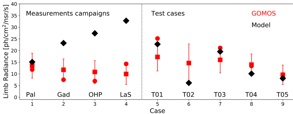
Fig. 6. In red squares are represented OH(8–4) integrated limb radiances from GOMOS between 925 nm and 955 nm averaged within a month and \pm 15^\circ latitude for several cases. Corresponding simulations are associated with the black diamonds and the closest observations are in red circles.
