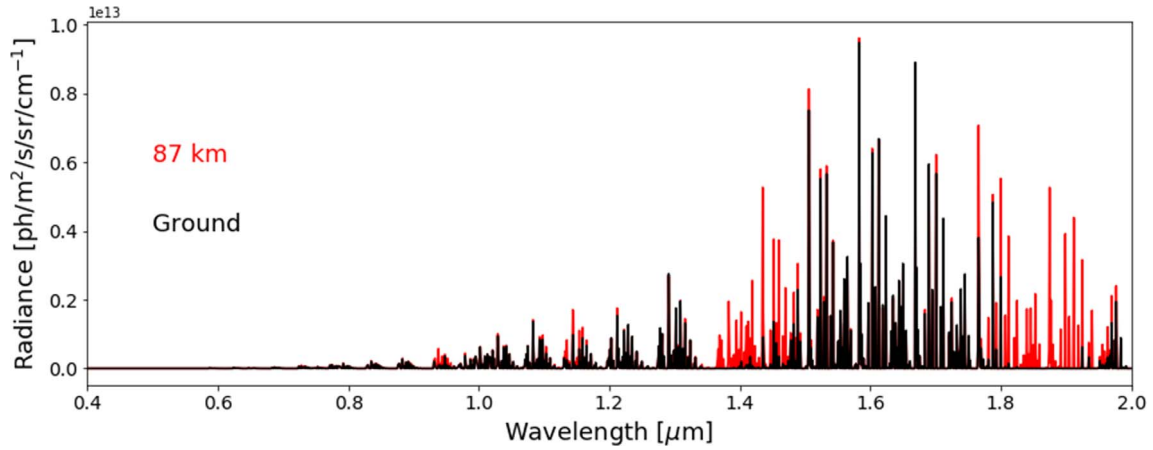
Fig. 1. Example of a spectrum at 87 km (in red) and the same spectrum propagated at the ground level (in black). We notice the strong water vapor absorption band around 1.4 \mu\text{m} .
