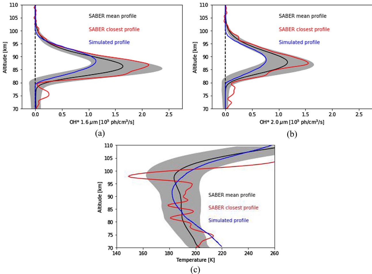
Fig. 5. (a) OH 1.6 μm profiles from simulation (in blue), and observations (mean profile in black and closest profile in red). The \pm 1 standard deviation from the mean is represented with the grey shade. (b) Same as (a) but for OH 2.0 μm. (c) Associated temperature profiles. The simulated temperature profile originates from MSIS data.
