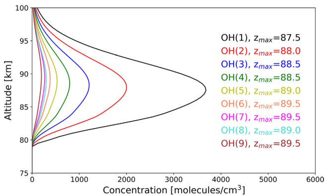
Fig. 3. Examples of OH vibrational states concentration as function of altitude.
