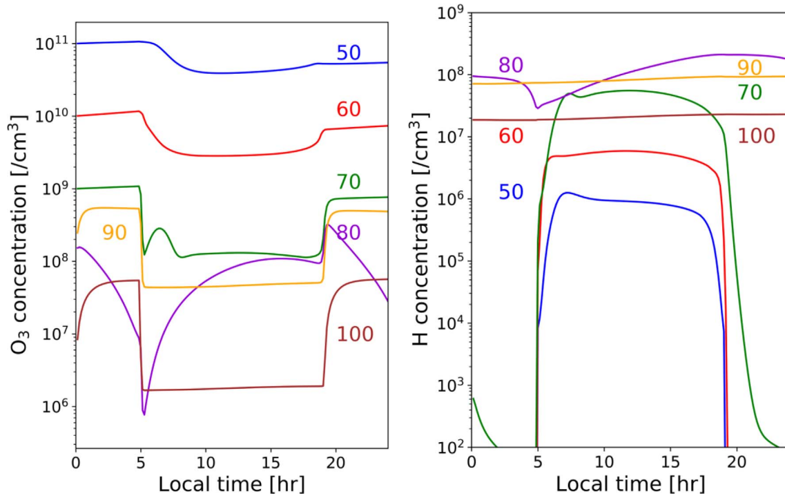
Fig. 2. Examples of molecules concentration evolution, O 3 on the left and H on the right. Ozone is strongly dependent on the solar cycle above 60 km. Below 80 km, H originates from the water vapor dissociation.
