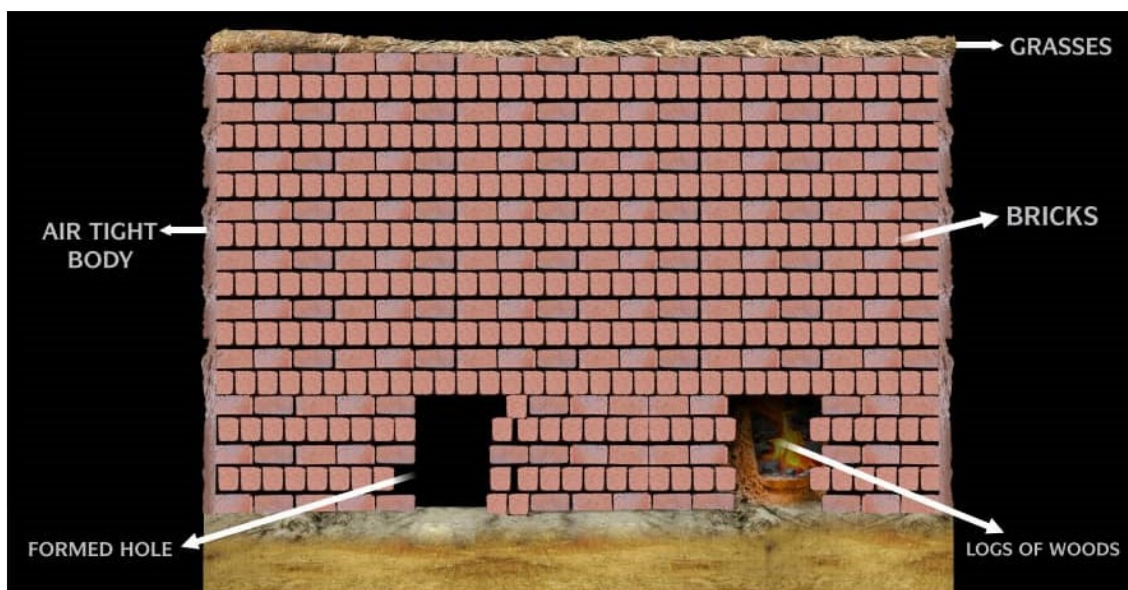
Figure 6: Cross-section of Final Kiln for Baking Burnt Bricks
