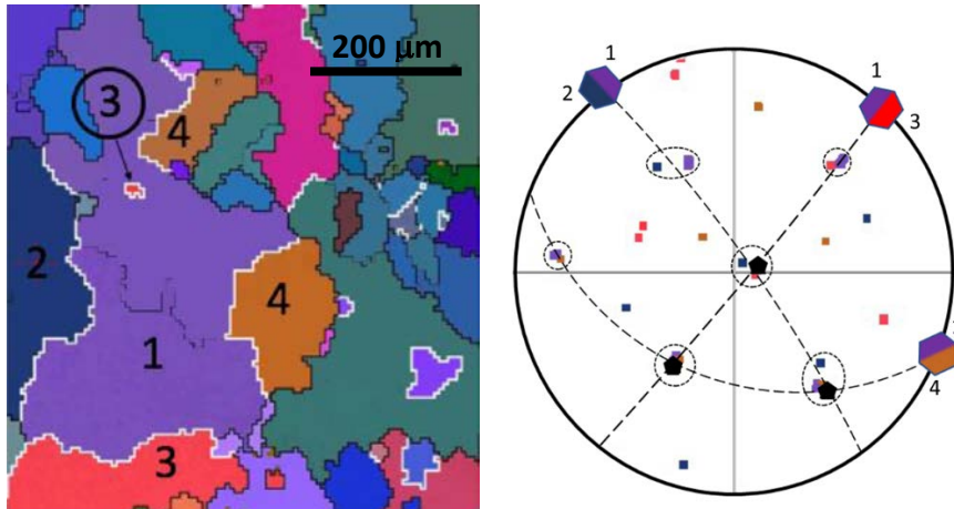
Figure 7: EBSD false color grain structure of Au-12.5wt.%Cu-12.5wt.%Ag with 2% Al 2 Yb addition to the melt. Twin grain boundaries are indicated in white. The \langle 110 \rangle pole figure of grains 1-4 are shown on the right with the common \{111\} plane between 1-2, 1-3 and 1-4 indicated by dashed arcs of circle. The common \langle 110 \rangle directions are circled. At the crossing of common \{111\} twin planes, there are 3 common \langle 110 \rangle directions for grains 1-2-3, 1-2-4 and 1-3-4 and the small pentagons correspond to the calculated position of three of the 5-fold axes of an icosahedron (adapted from [36]).
