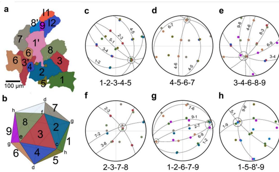
Figure 5: (a) EBSD false-color grain structure maps of 9 grains in Au-12.5wt.%Cu-12.5wt.%Ag with 20 ppm Ir. The \langle 110 \rangle pole figures of sets of MT grains are shown in (c-h), with the common \langle 110 \rangle direction circled in each figure and indication of the \{111\} twin or near-twin planes by arcs of circle. In (b), an icosahedron has been schematically drawn in a position such that the six 5-fold symmetry axes labeled (c-h) approximately correspond to the common \langle 110 \rangle axes of the fcc grains, and with corresponding facets of the same color as grains in (a) (adapted from [29]).
