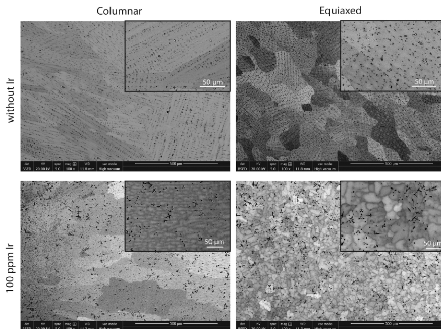
Figure 9: SEM-BSE images Au-20.5wt.%Cu-4.5wt.%Ag without (top) and with (bottom) 100 ppm of Ir added to the melt. The small droplet of each alloy has been solidified rapidly on a Cu substrate, producing a columnar structure close to the chill (left) and equiaxed grains near the top (right) [37]. The small inserts show magnification of the microstructure. Black dots correspond to Cu-rich dendrites/particles, while Au-rich grains appear with various grey levels.
