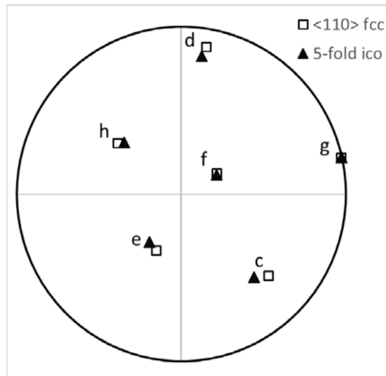
Figure 6: Stereographic projection corresponding to the pole figures of Figure 5, where the common \langle 110 \rangle directions seen in (c-h) are shown as open squares. The filled triangles have been calculated from the directions of the 5-fold symmetry axes of an icosahedron, with an exact correspondence between \langle 110 \rangle_{fcc} and \langle 5\text{-fold axis} \rangle_{ico} for (g) and the best agreement for the other \langle 5\text{-fold axes} \rangle_{ico} directions.
