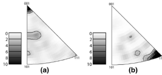
Figure 10: Inverse texture pole figures of the columnar zones in Au-20.5wt.%Cu-4.5wt.%Ag (Figure 9) without (a) and with (b) 100 ppm Ir [37]. In this unit triangle of the fcc structure, the color index corresponds to the probability to have the thermal gradient aligned with an \langle hkl \rangle direction of the columnar grains.
