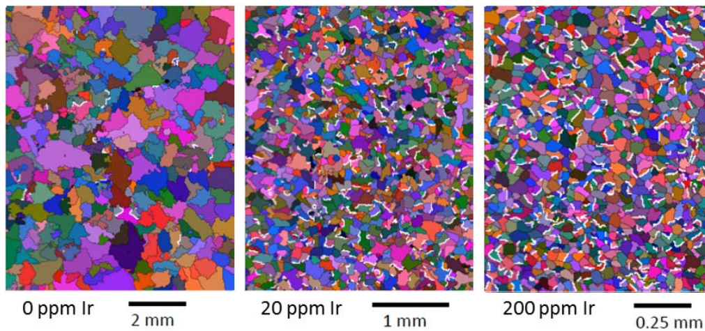
Figure 4: EBSD false-color grain structure maps of Au-12.5wt.%Cu-12.5wt.%Ag with various additions of Ir. Twinned grain boundaries detected with an accuracy of 5 deg. are shown in white (adapted from [29]).
