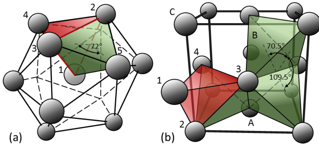
Figure 1: (a) Icosahedron with two nearest-neighbors of its 20 tetrahedra shown in red and green; (b) Unit cell of the fcc structure with representation of three of the 8 tetrahedra made of {111} planes and <110> edges (in green) and one stacking-fault induced by the attachment of one tetrahedron (in red).
