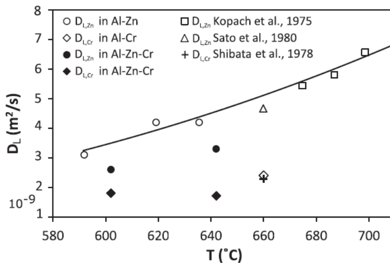
Figure 11: Diffusion coefficients of Zn and Cr in the liquid for Al-Zn and Al-Zn-0.1wt.%Cr alloys as measured from the solute profile in the quenched liquid ahead of a planar-front during Bridgman solidification [40].
