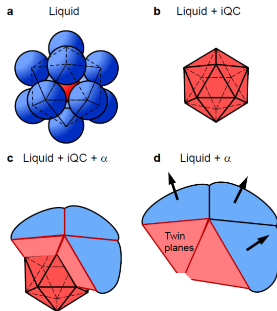
Figure 3: Schematic representation of the ISRO- or iQC-mediated nucleation mechanism: (a) formation of ISRO in the liquid; (b) formation of iQC on which (c) the fcc phase can form with heteroepitaxy relationships with the icosahedron, producing MT grains; (d) further growth of the fcc phase and disappearance of the iQC template by peritectic transformation [29].
