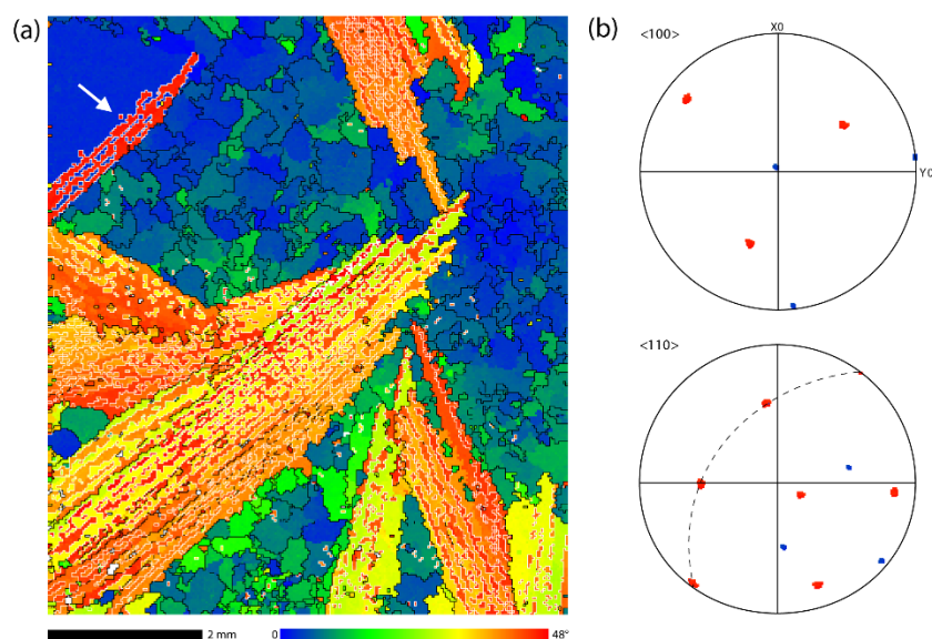
Figure 13: (a) EBSD false color map of a transverse section of an Al-4.3wt.%Cu-0.3wt.%Mg directionally solidified sample, taken 6 mm from the chill surface (redrawn from data coming from
