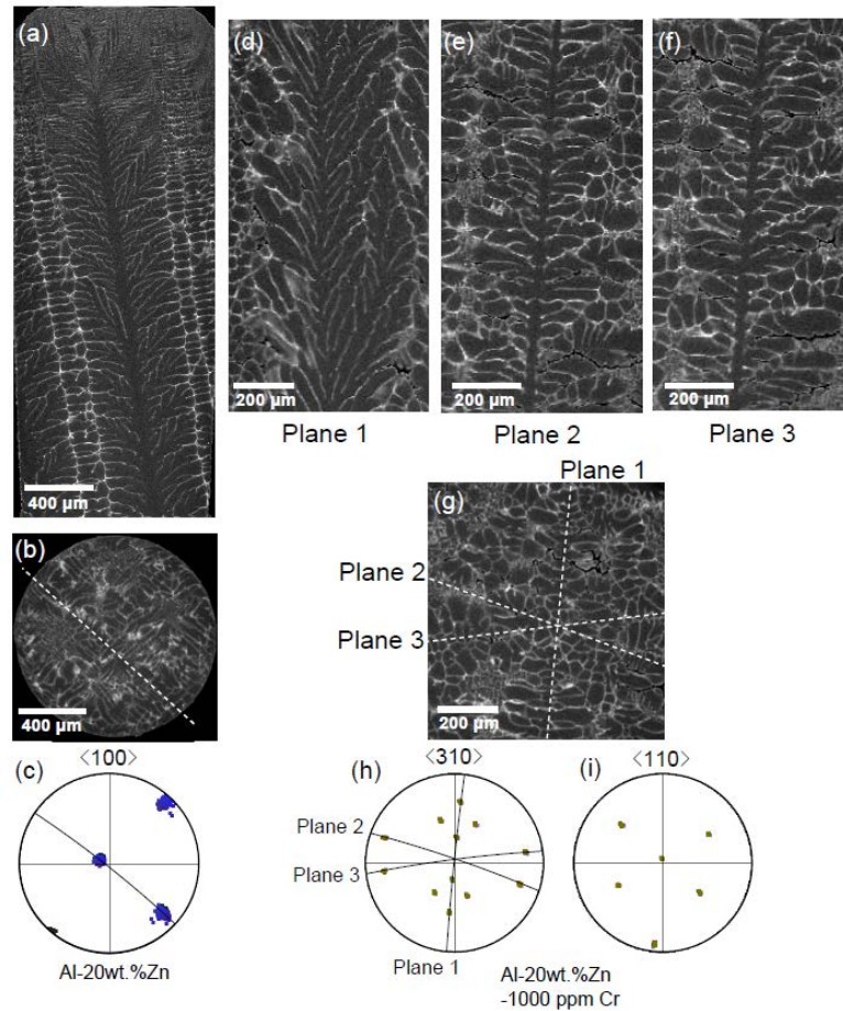
Figure 8: 2-dimensional views of X-ray microtomography analyses of Al-20wt.%Zn alloys solidified in a Bridgman furnace at 67 \mu\text{m/s} in a 100 \text{ K/cm} thermal gradient, (a-c) without Cr, (d-i) with 0.1wt.%Cr. (a) and (d-f) correspond to longitudinal sections, (b) and (g) to transverse sections and (c), (h) and (i) are relevant pole figures corresponding to the transverse sections (i.e., thermal gradient located at the center) [28].
