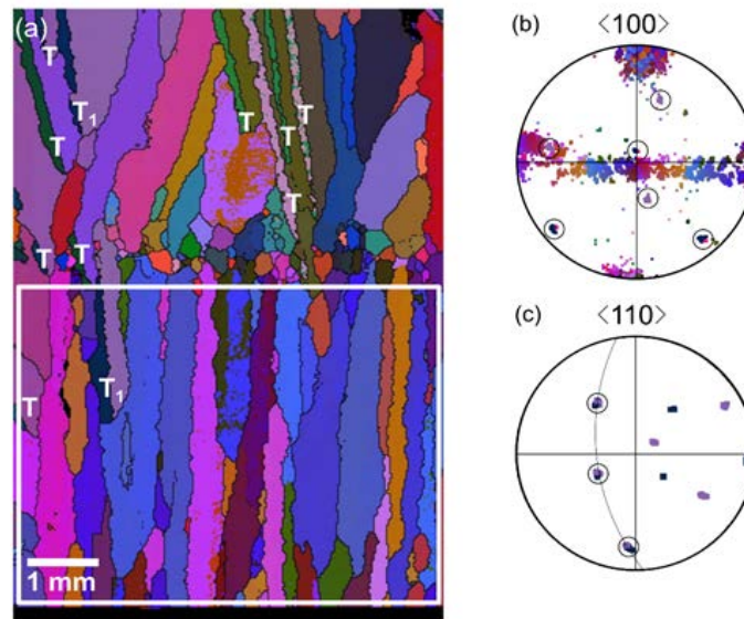
Figure 12: (a) EBSD false color map of a longitudinal section of an Al-20wt.%Zn-0.1wt.%Cr specimen directionally solidified. Regular dendritic grains at the bottom exhibit a \langle 100 \rangle texture, as shown in (b), while the \langle 110 \rangle pole figure in (c) is for the isolated twinned dendrites labelled "T 1 ". Other twinned dendrites in the upper part of the specimen are clearly visible.[38]
