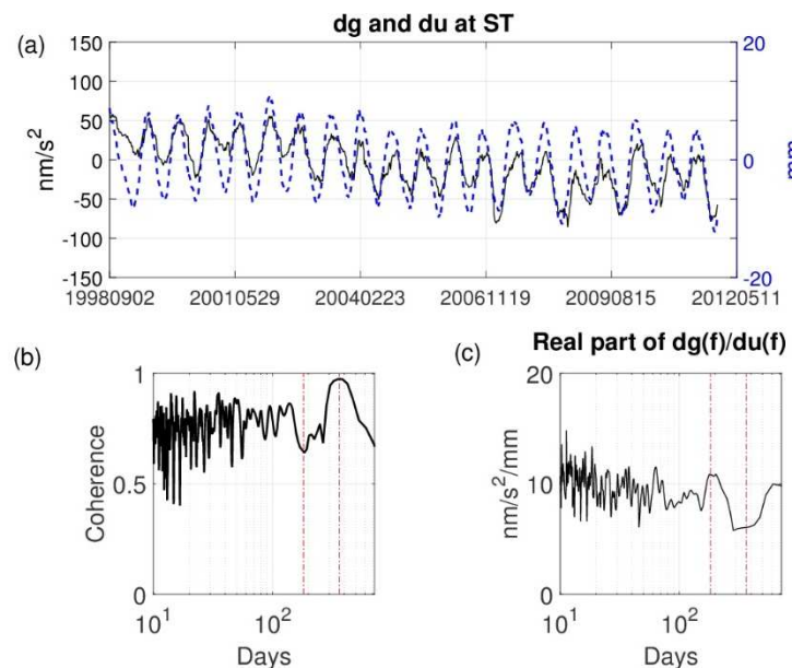
Fig. 3 Total surface loading gravity and vertical changes predicted at Strasbourg (France) from MERRA2 hydrological model. (a) dg (black line) and du (dashed blue line) surface loading time-series; (b) magnitude squared coherence; (c) real part of the transfer function between dg and du . Vertical dashed red lines indicate the annual and semi-annual periods.
