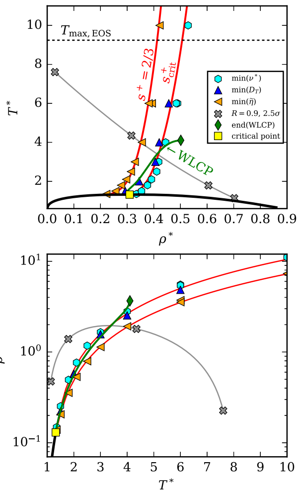
FIG. 5. The curves s^+ = 2/3 and s^+_{crit} and WLCP for the full L-J fluid, each evaluated from the EOS of Thol et al. [36] with T^*_{crit} = 1.32 and \rho^*_{crit} = 0.31 at the critical point in T - \rho (upper) and p - T coordinates (lower). The thick black curve is the binodal, and the grey line is a smoothed curve fit to the interpolated R=0.9 points. The minima of \tilde{\eta} and \nu^* are taken from interpolations of the equilibrium molecular dynamics simulations of Ref. 26 for the nominal isotherms of T^*=(1.35,1.5,1.8,2.1,2.5,3,4,6) , and from non-equilibrium simulations in this work for T^*=(6,10) (tabular results in the SI, Table S3). The minima of D_T were taken from the non-equilibrium simulations of Ref. 48 for nominal isotherms of T^*=(2,3,4,6) .
