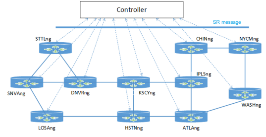
Fig. 3: A depiction of the experimental SDN-based SR Abilene topology network
