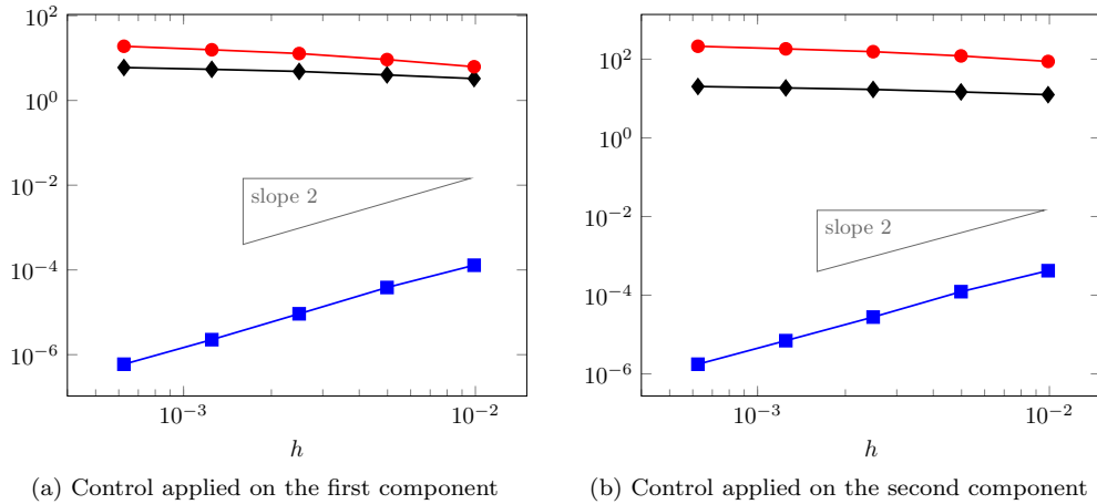
FIG. 11. Convergence properties of the HUM technique with Neumann control applied in different equations for a = 2, \alpha = 4 (the systems (1.7)–(5.22)). Same legend as in Figure 6.
