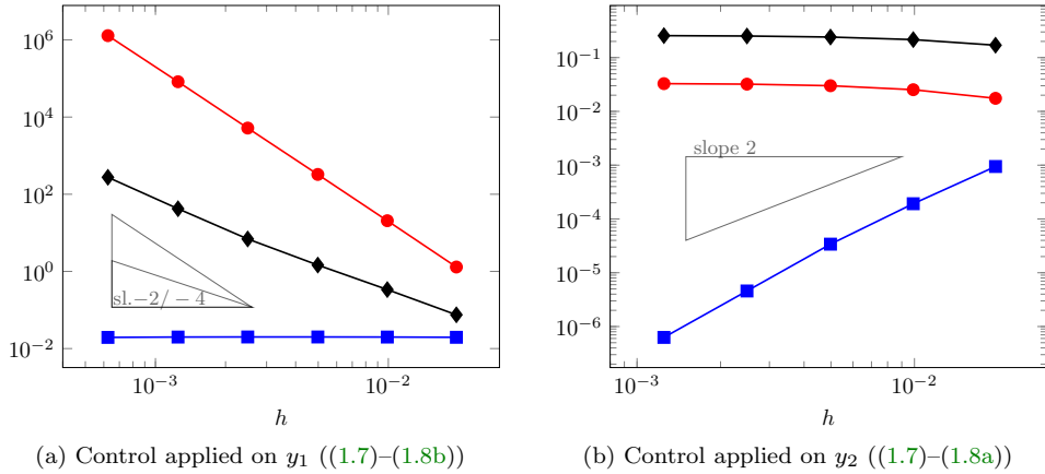
FIG. 8. Convergence properties of the HUM technique for the critical pair (\alpha_0, a_0) with Dirichlet control applied on different components. Same legend as in Figure 6.
