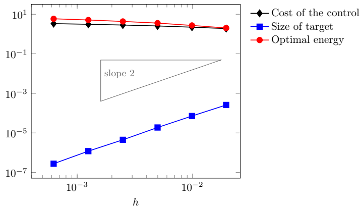
FIG. 6. Convergence properties using the penalized HUM technique, the case a = 0, \alpha = 1 (Dirichlet control case).
