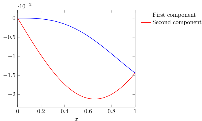
FIG. 7. The eigenfunction \Phi_{\lambda_{\alpha_0, a_0}^c} corresponding to the critical eigenvalue \lambda_{\alpha_0, a_0}^c (Dirichlet case).
