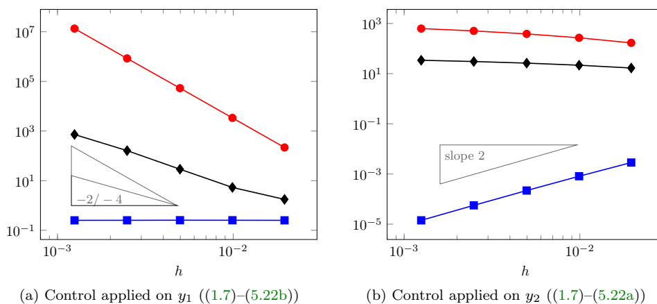
FIG. 14. Convergence properties w.r.t. HUM approach for the critical pair (\alpha_c, a_c) with Neumann control applied on different components.
