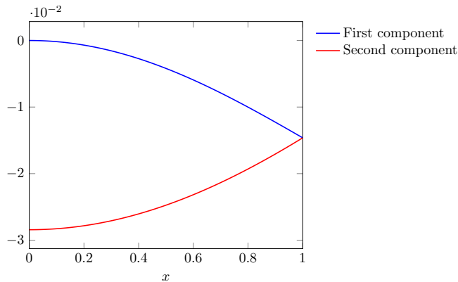
FIG. 13. The eigenfunction \Phi_{\lambda_{\alpha_c, a_c}^1} corresponding to the critical eigenvalue (the first one) \lambda_{\alpha_c, a_c}^1 (Neumann case).
