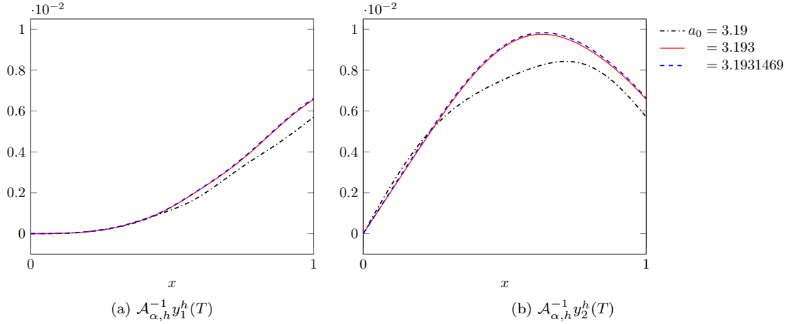
FIG. 10. Convergence of the target for \alpha_0 = 1 and different approximations of a_0 for the system (1.7)–(1.8b).
