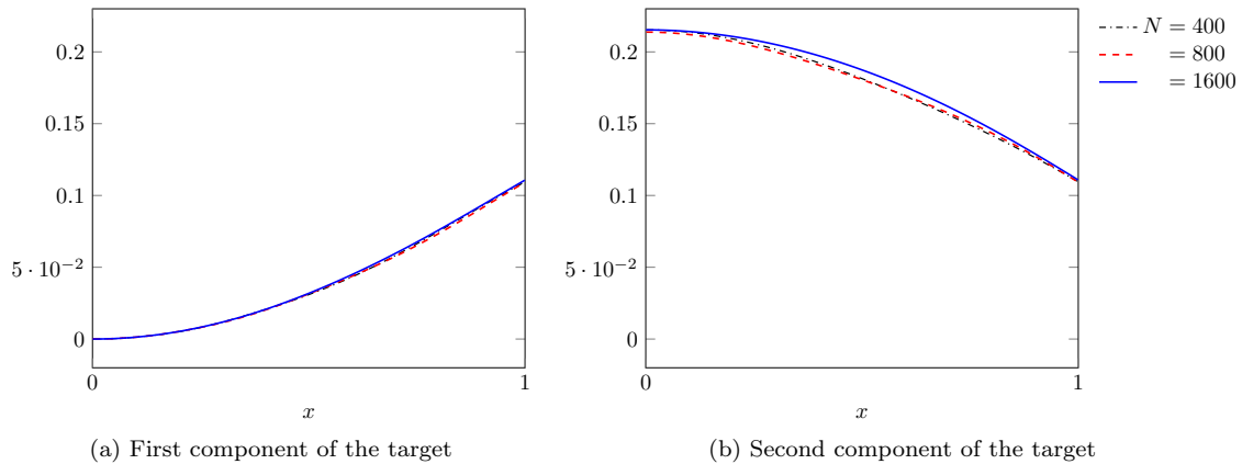
FIG. 15. Convergence of the target as h \downarrow 0 for the critical values (\alpha_c, a_c) = (0.1, 1.2369289) for the system (1.7)–(5.22b).
