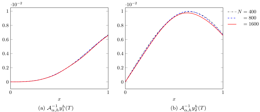
FIG. 9. Convergence of the target as h \downarrow 0 for the critical pair (\alpha_0, a_0) = (1, 3.1931469) for the system (1.7)–(1.8b).
