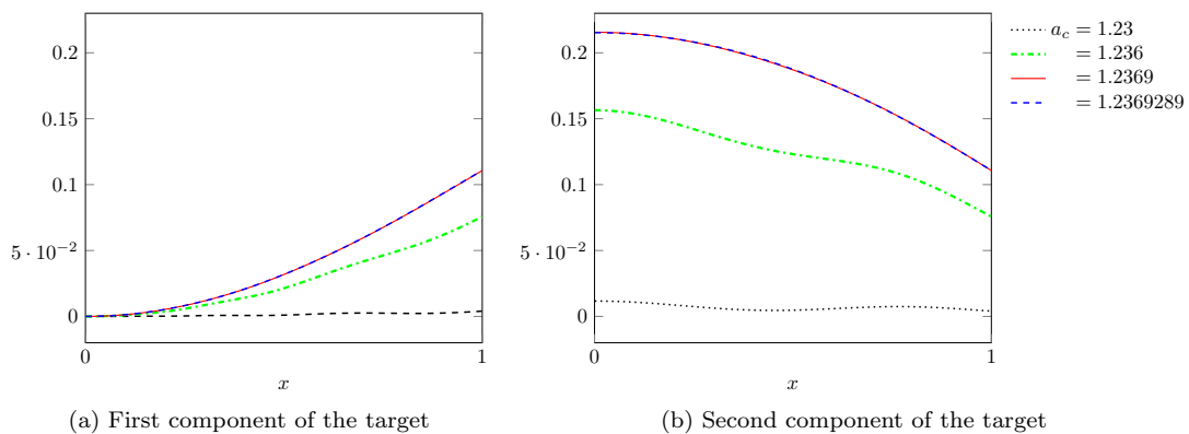
FIG. 16. Convergence of the target for \alpha_c = 0.1 and different approximations of a_c for the system (1.7)–(5.22b).
