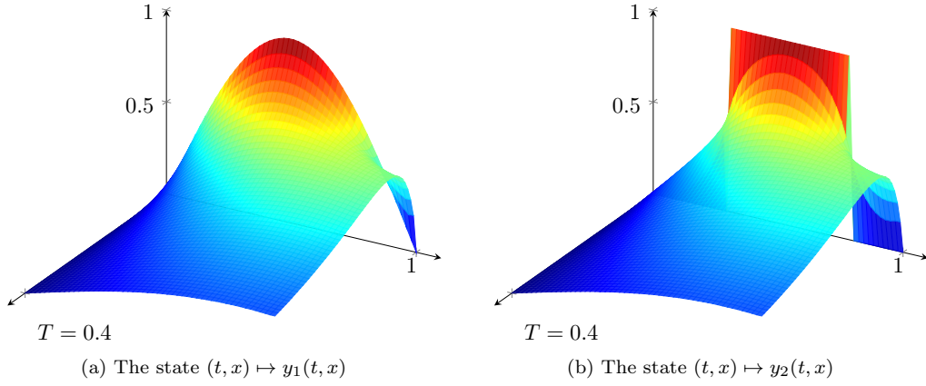
FIG. 3. Evolution in time of the uncontrolled solution of system (1.7)–(1.8b) for a = 0, \alpha = 1 .
