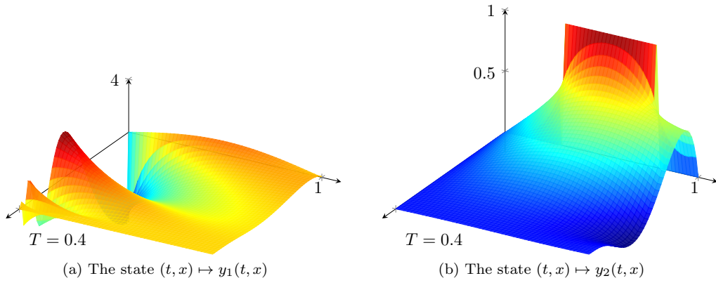
FIG. 4. Evolution in time of the controlled solution of system (1.7)–(1.8b) for a = 0, \alpha = 1 .
