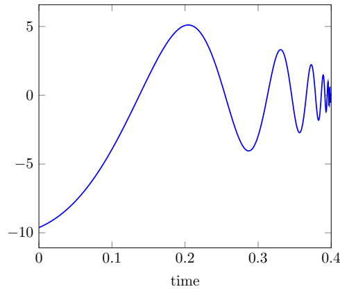
FIG. 5. Control function v(t) .
