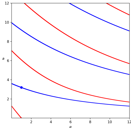
FIG. 2. In blue: the set \mathcal{R} of critical pairs (\alpha, a) . In red: The solutions to (4.28b) that are not solution of (4.28a).
