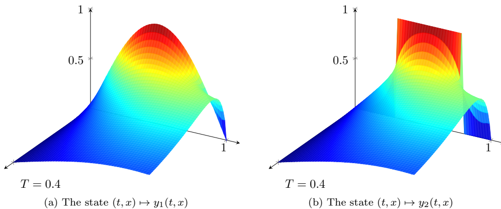
FIG. 3. Evolution in time of the uncontrolled solution of system (1.8)–(1.9b).
