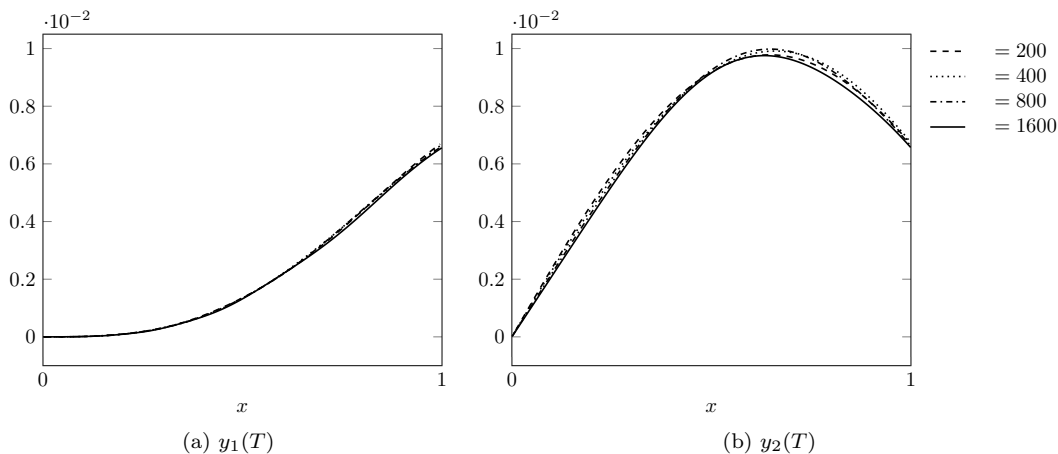
FIG. 9. Convergence of the A_{\alpha,h}^{-1} y^h(T) as h \downarrow 0 .
