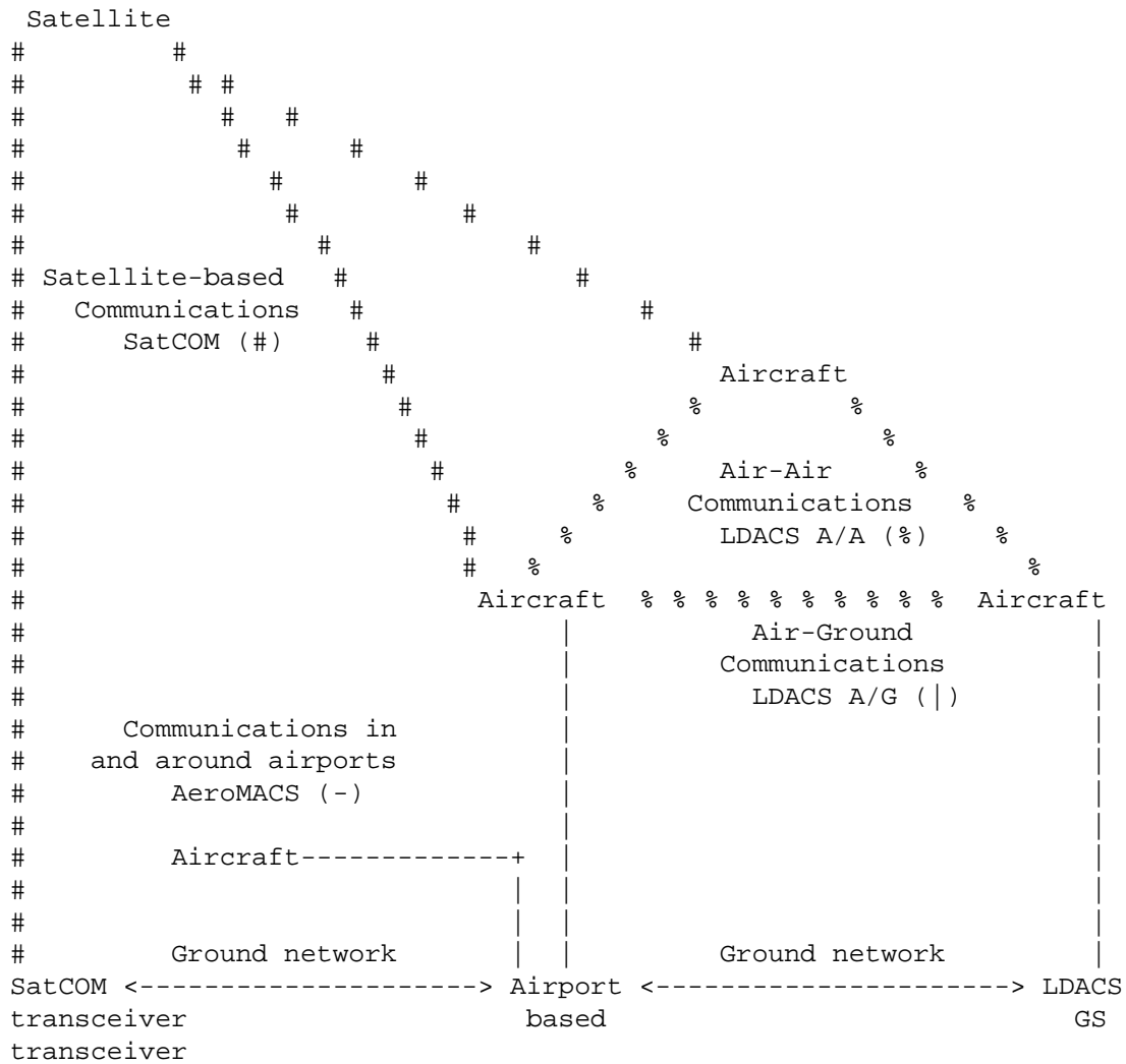
Figure 1: The Future Communication Infrastructure (FCI): AeroMACS for APT/TMA domain, LDACS A/G for TMA/ENR domain, LDACS A/G for ENR/ORP domain, SatCOM for ORP domain communications
