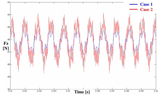
Figure 14: Dynamic load Fz on bearing B5 (cases 1 & 2)
