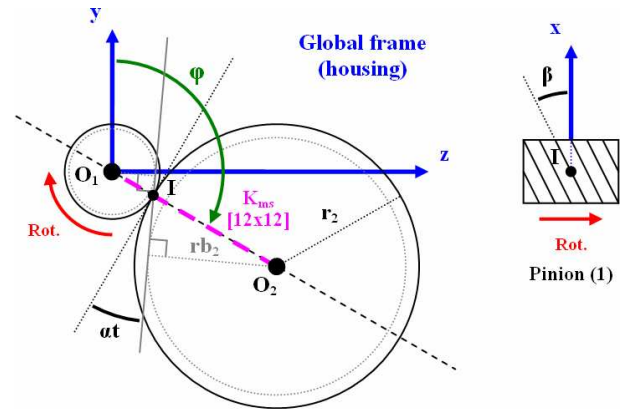
Pinion (1) and wheel (2) in transverse plane
