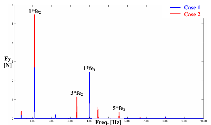
Figure 16: Magnitude spectrum of Fy on bearing B5
