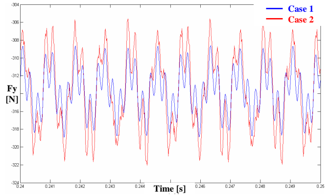
Figure 13: Dynamic load Fy on bearing B5 (cases 1 & 2)
