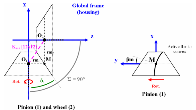
Figure 8: Spiral bevel gears in the global frame
