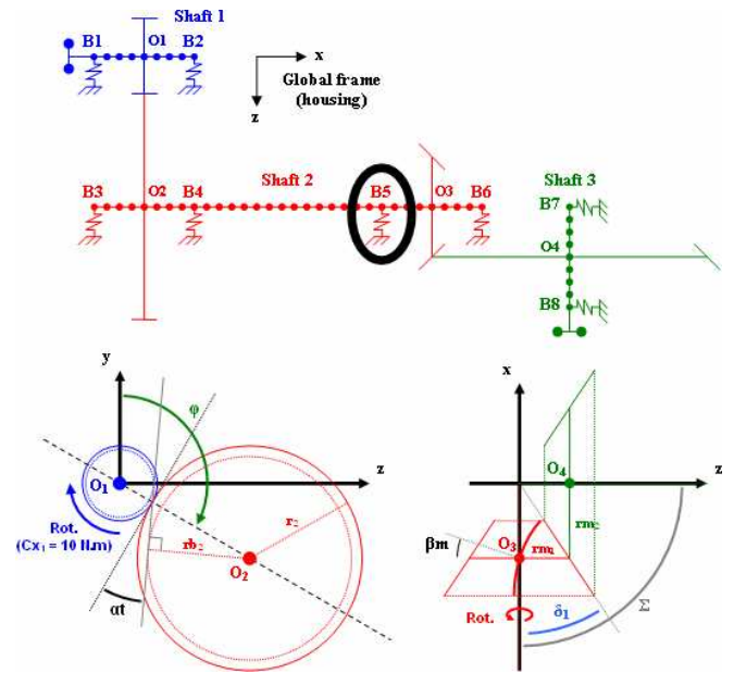
Figure 9: Transmission system with two gear pairs
