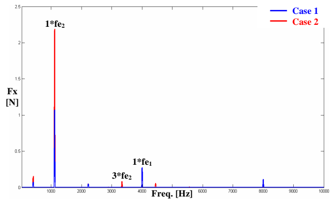
Figure 15: Magnitude spectrum of Fx on bearing B5
