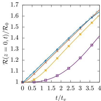
FIG. 14: Evolution of the filament radius in the midplane z = 0 for \text{Oh} = 10 . -\text{+}- : \mathcal{A} = 5 , -\text{x}- : \mathcal{A} = 10 , -\text{*}- : \mathcal{A} = 20 , -\square- : \mathcal{A} = 40 , --- : theoretical prediction (24).
