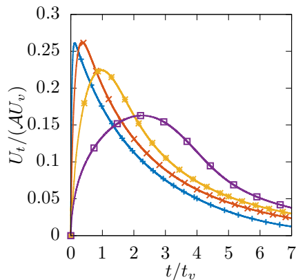
FIG. 12: Tip velocity vs. time for Oh = 10 and different initial aspect ratios. \cdot -\text{+}- : \mathcal{A} = 5 , -\times- : \mathcal{A} = 10 , -\ast- : \mathcal{A} = 20 , -\square- : \mathcal{A} = 40 .
