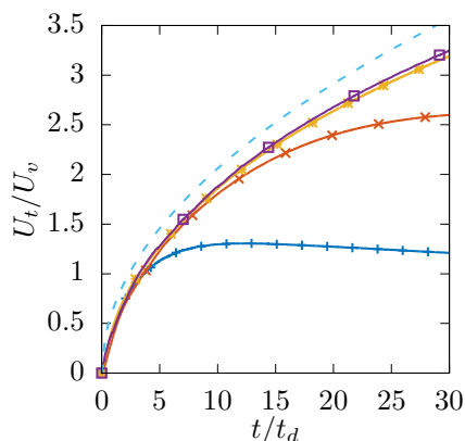
FIG. 11: Tip velocity vs. time for \text{Oh} = 10 and different initial aspect ratios during the initial transient. -\text{+}- : \mathcal{A} = 5 , -\times- : \mathcal{A} = 10 , -*- : \mathcal{A} = 20 , -\square- : \mathcal{A} = 40 , --- : prediction (22).
