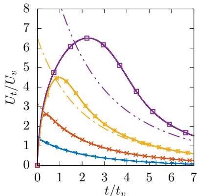
FIG. 15: Evolution of the tip velocity for \text{Oh} = 10 . -\text{+}- : \mathcal{A} = 5 , -\text{x}- : \mathcal{A} = 10 , -\text{*}- : \mathcal{A} = 20 , -\square- : \mathcal{A} = 40 ; dotted lines: theoretical prediction (25).
