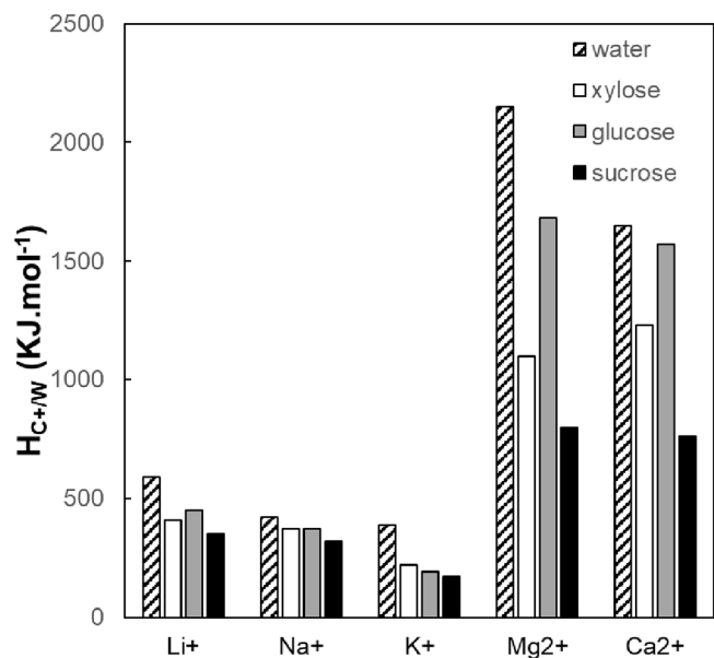
Fig. 2. Cation enthalpy hydration, H_{\text{C}^+/\text{W}} of \text{Li}^+ , \text{Na}^+ , \text{K}^+ , \text{Mg}^{2+} , \text{Ca}^{2+} in pure water and in presence of saccharides (in absolute value)/water molecules, at 298.15 K.
