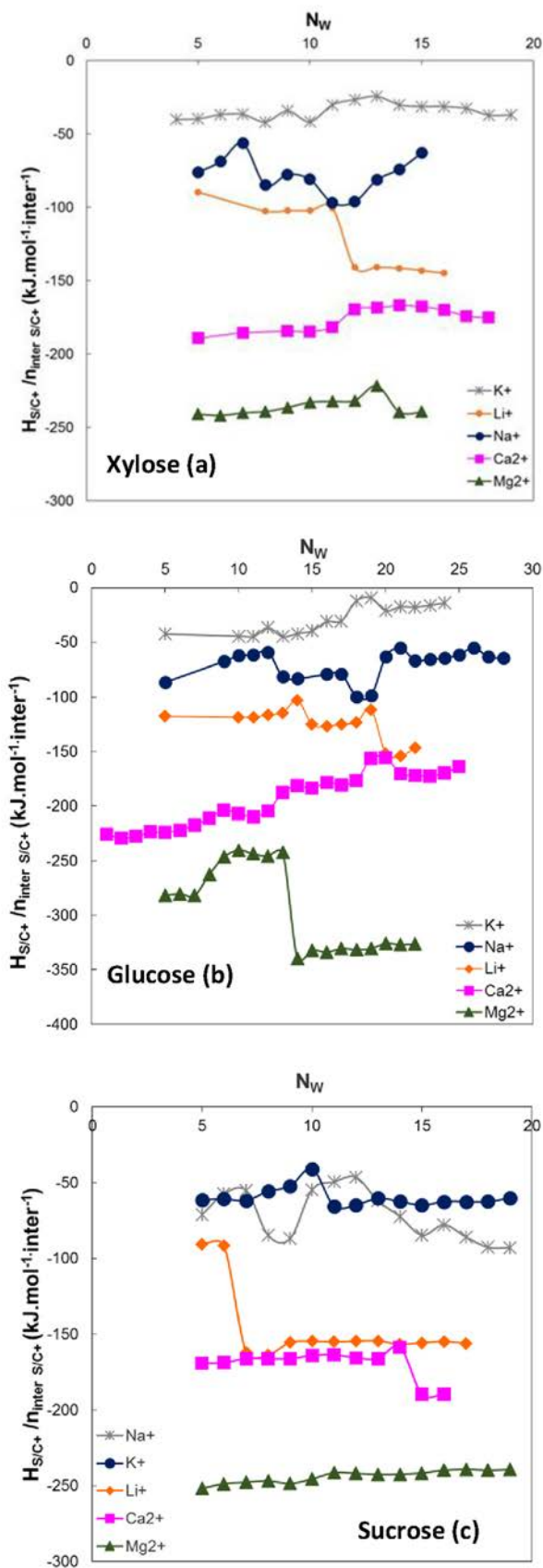
Fig. 4. Variation of saccharide/cation interaction enthalpy, related to the number of saccharide/cation interactions, H_{S/C+}/n_{inter\ S/C+} , as function of the water molecules number N_w , at 298.15 K: Influence of the nature of the cation. Xylose (a), Glucose (b), Sucrose (c).
