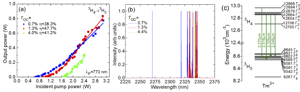
Fig. 8. Tm:KY 3 F 10 laser operating at the 3 H 4 → 3 H 5 transition: (a) input-output dependences, \eta – slope efficiency; (b) typical laser emission spectra. The laser emission is unpolarized, \lambda_p = 773 nm; (c) details of the Stark splitting of the upper and lower laser levels showing the observed laser transitions (green arrows), \Gamma_i are the irreducible representations.
