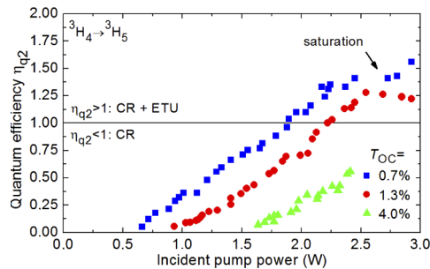
Fig. 11. Calculated pump quantum efficiency \eta_{q2} for the Tm:KY 3 F 10 laser operating at the {}^3\text{H}_4 \rightarrow {}^3\text{H}_5 transition ( \lambda_p = 773 nm). Intracavity roundtrip losses: 2L = 0.7\% .
