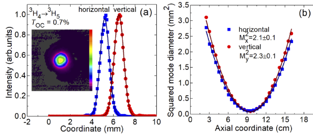
Fig. 10. Output laser beam of the Tm:KY 3 F 10 laser operating at the 3 H 4 → 3 H 5 transition: (a) 1D intensity profiles along the horizontal and vertical directions (symbols) and their Gaussian fits (curves), inset – 2D mode profile, far-field; (b) evaluation of the beam quality factors M^2_{x,y} . \lambda_p = 773 nm, P_{inc} = 1.7 W, T_{OC} = 0.7\% .
