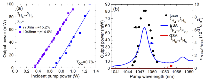
Fig. 12. Upconversion-pumped Tm:KY 3 F 10 laser operating at the {}^3\text{H}_4 \rightarrow {}^3\text{H}_5 transition: (a) input-output dependence, \eta – slope efficiency, \lambda_p = 1048 nm. The results for conventional pumping ( \lambda_p = 773 nm) are given for comparison. T_{OC} = 0.7\% ; (b) laser excitation curve: circles – output power of the laser ( P_{inc} = 0.92 W, T_{OC} = 0.7\% ), blue and red curves – parts of the ESA and GSA cross-section spectra for the {}^3\text{F}_4 \rightarrow {}^3\text{F}_{2,3} and {}^3\text{H}_4 \rightarrow {}^3\text{H}_5 transitions, respectively.
