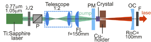
Fig. 5. Scheme of the Tm:KY 3 F 10 laser: P – Glan-Taylor polarizer, \lambda/2 – rotatory half-wave plate, TL – telescope, FL – focusing lens, PM – pump mirror, OC – output coupler, F – band-pass filter.
