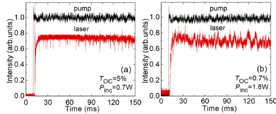
Fig. 6. Typical oscilloscope traces of incident pump and laser emission for the Tm:KY 3 F 10 laser: operation at (a) {}^3F_4 \rightarrow {}^3H_6 and (b) {}^3H_4 \rightarrow {}^3H_5 transitions. \lambda_P = 773 \text{ nm} .
