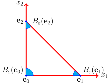
Figure 5: Domain B_\varepsilon(\mathbf{e}_i)
