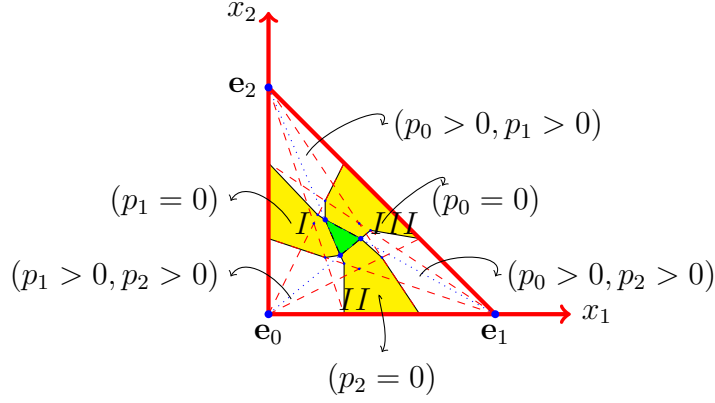
Figure 8: K_1 = \text{white domains} + \text{yellow domains} = \Delta_2 - \text{green domain} ; K_1^c is green domain; \Omega_1(1), \Omega_2(1), \Omega_0(1) are yellow domains I, II, III correspondingly.
