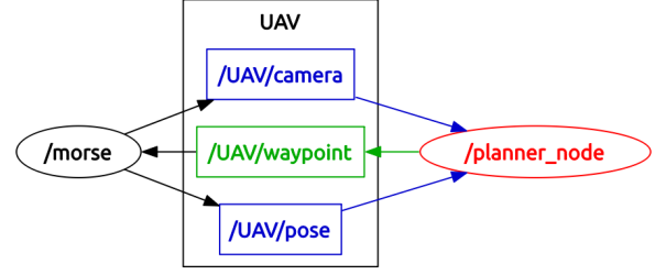
Figure 3: Graph of the ROS nodes interacting during a simulation. The communication with the sensors and the actuators happens via messages, here indicated as camera , waypoint (the destination plot), and pose (the current position of the UAV). Data are processed in nodes morse (simulation) and planner_node (planning).
