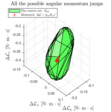
(f) Angular momentum
