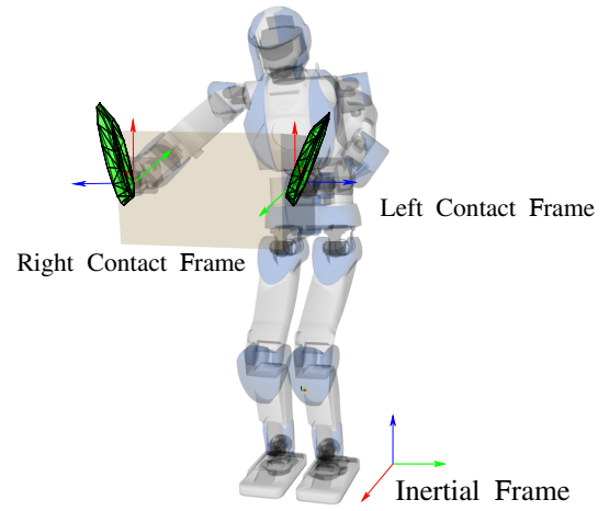
Figure 9. We color x , y and z axes with red, green and blue, respectively. The two green polyhedra align with the two contact frames, representing the impulse sets \mathcal{X}_i for the two arms during the second grabbing. It should be noted that the scale of the polyhedra does not correspond to the robot's geometry.
