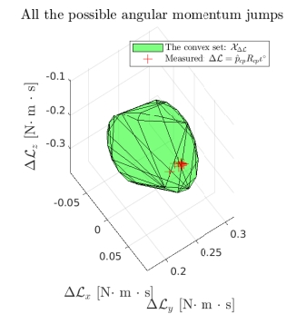
(f) Angular momentum
