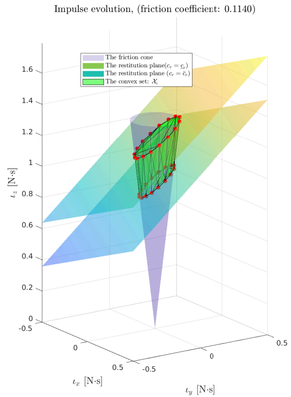
Figure 4. We visualize the impulse set \mathcal{X}_l when the Panda manipulator in Fig. 6(a) impacted at contact velocity \mathbf{v} = [-0.0001, -0.0117, 0.174] m/s (in the contact point frame). In comparison to Fig. 3, the reduction in friction coefficient from 0.279 to 0.114 leads to a narrower impulse set \mathcal{X}_l .
