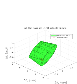
(e) COM velocity
