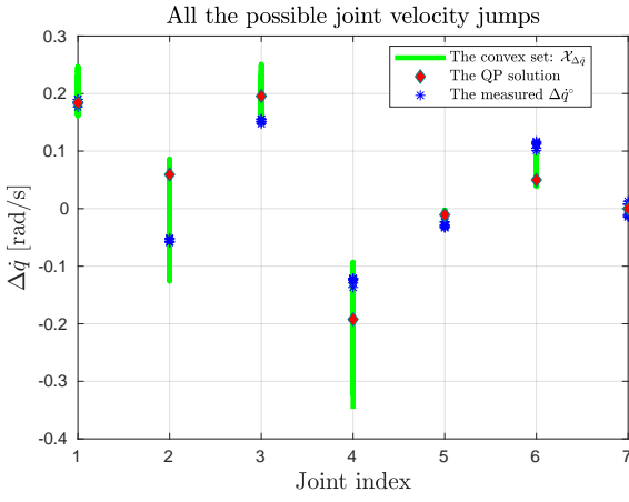
Figure 7. The measured and predicted joint velocity jumps of the Panda manipulator during different trials of Experiment 1 . The inequality constraint (29) was inactive as the post-impact joint velocities remained well within the bounds defined by (37).
