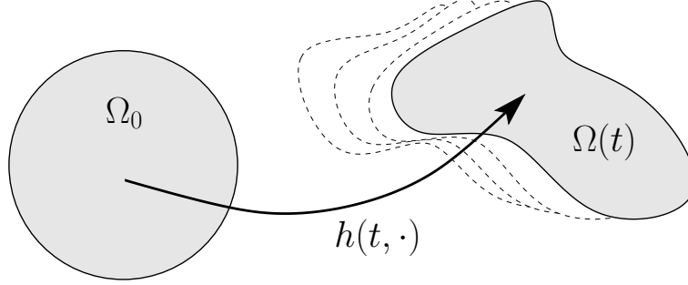
Figure 1: The family of diffeomorphisms (h(t, \cdot))_{t \in I} which enables to go back to a fixed domain \Omega_0 .
