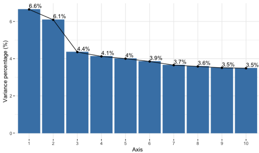
FIG 6.: MCA spatial analysis, Doubs department: variance percentage on the first 10 axes.
