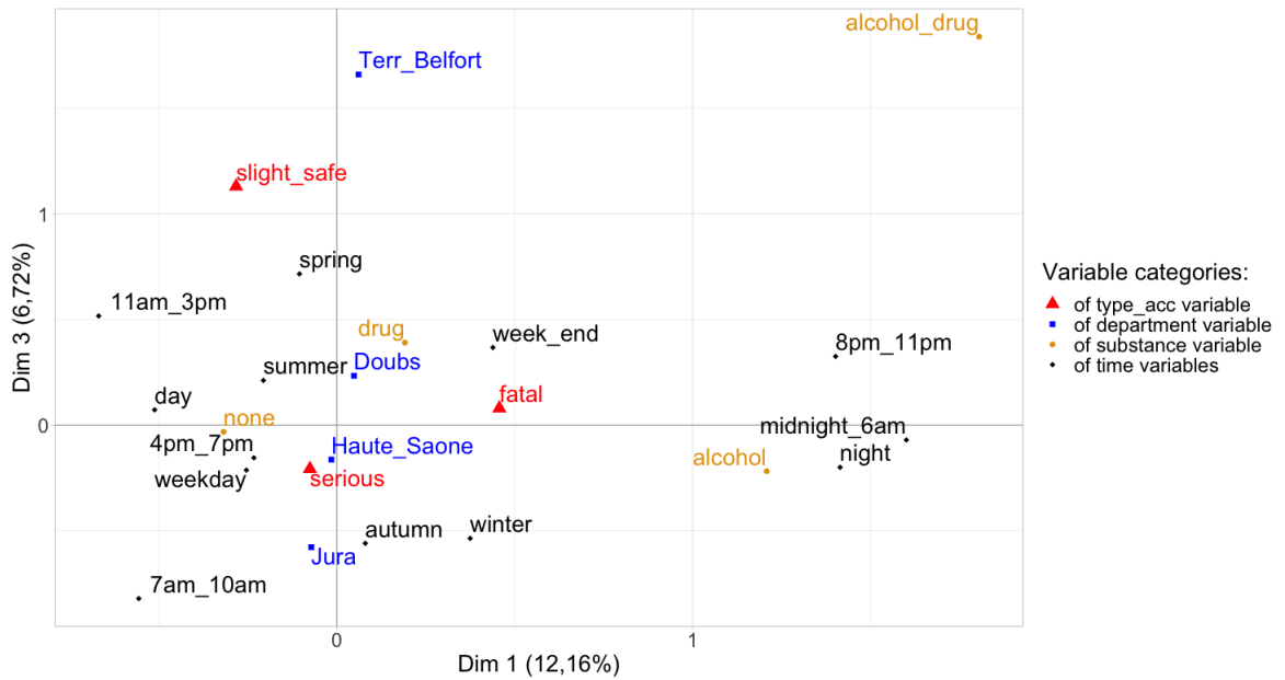
FIG 11.: MCA global analysis: factorial plane made by axis 1 and axis 3.
