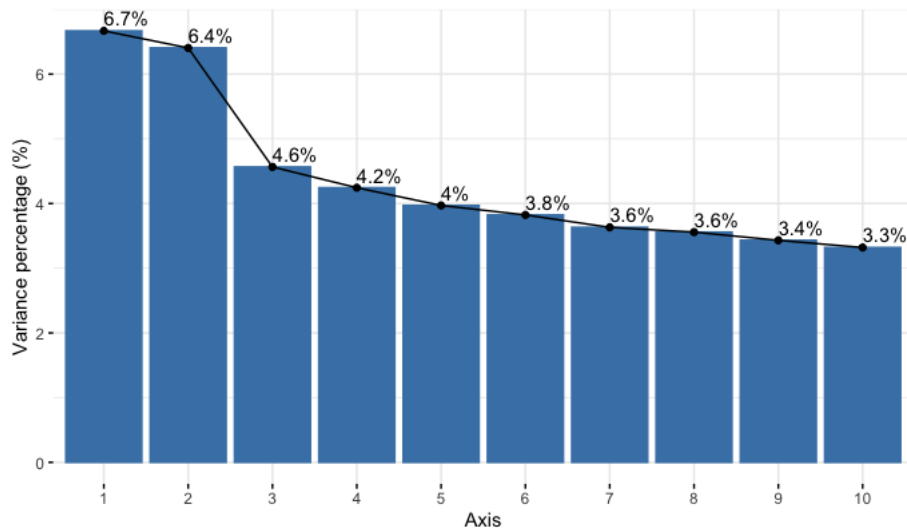
FIG 8.: MCA spatial analysis, Jura department: variance percentage on the first 10 axes.
