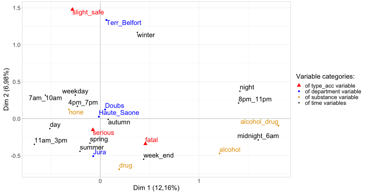
FIG 10.: MCA global analysis: factorial plane made by axis 1 and axis 2.
