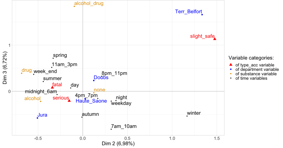
FIG 12.: MCA global analysis: factorial plane made by axis 2 and axis 3.
