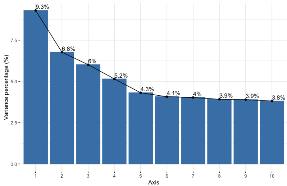
FIG 2.: MCA temporal analysis: variance percentage explained by the first 10 axes.
