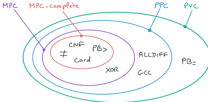
Figure 4: A classification of Constraints
