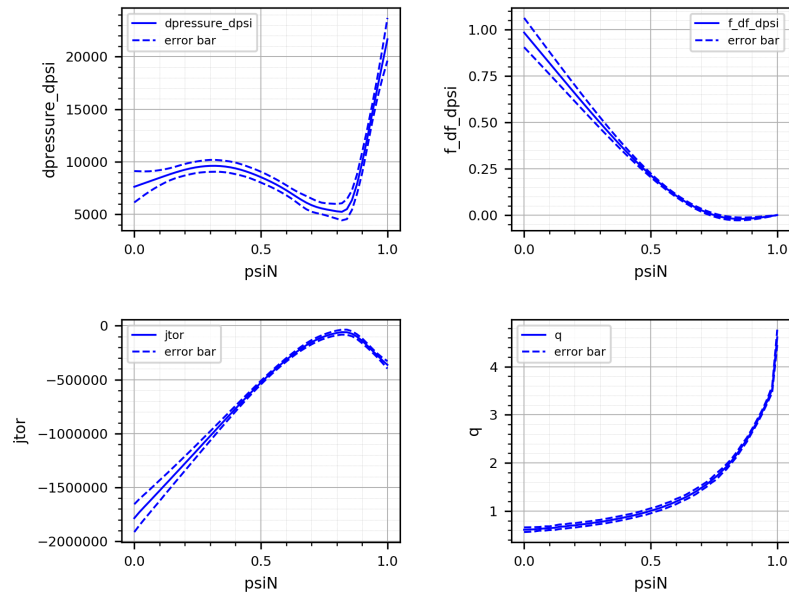
Figure 15: JET equilibrium reconstruction with magnetics and pressure. Reconstructed p' , f f' , j_{tor} = (p' + \langle 1/r^2 \rangle (1/\mu_0) f f') / \langle 1/r \rangle and safety factor q profiles, and associated computed error bars.
