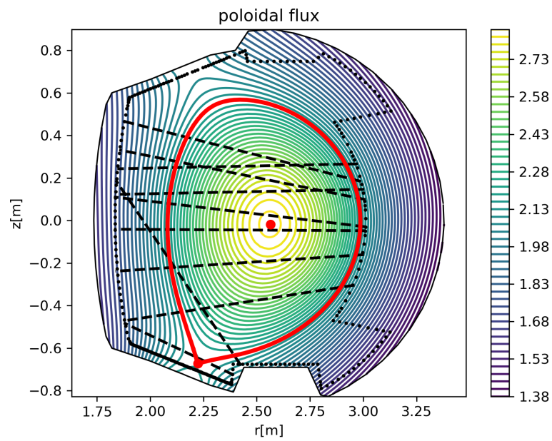
Figure 11: Poloidal flux map for a WEST equilibrium reconstruction with magnetics and interfero-polarimetry. The plasma boundary is shown in red. The limiter contour is the dotted line and the dashed lines are the interfero-polarimetry chords
