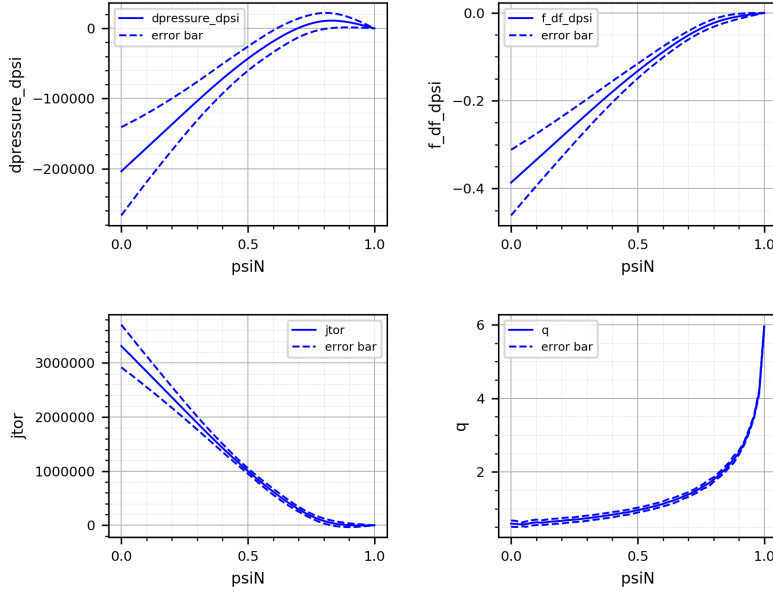
Figure 10: TCX equilibrium reconstruction with magnetics. Reconstructed p' , ff' , j_{tor} = (p' + \langle 1/r^2 \rangle (1/\mu_0)ff') / \langle 1/r \rangle and safety factor q profiles, and associated computed error bars.
