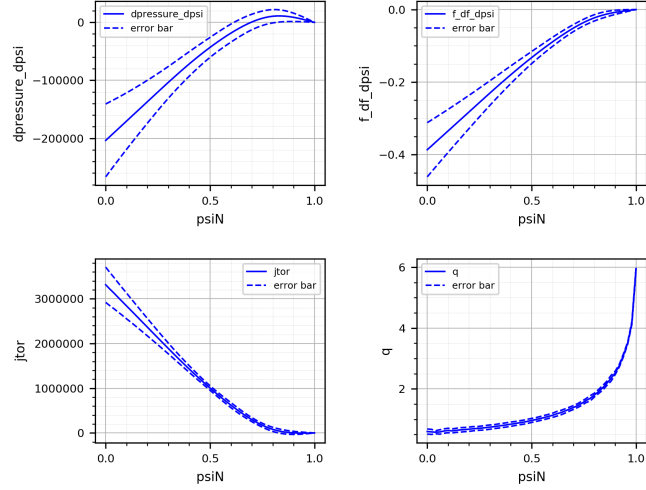
Figure 10: TCV equilibrium reconstruction with magnetics. Reconstructed p' , ff' , j_{tor} = (p' + \langle 1/r^2 \rangle (1/\mu_0)ff') / \langle 1/r \rangle and safety factor q profiles, and associated computed error bars.
