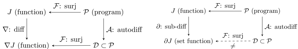
Figure 2: Left: Automatic differentiation applied to programs combining smooth functions in a smooth way, the diagram commutes. Right: Automatic differentiation in nonsmooth settings, no connection with known notion of generalized derivative.
