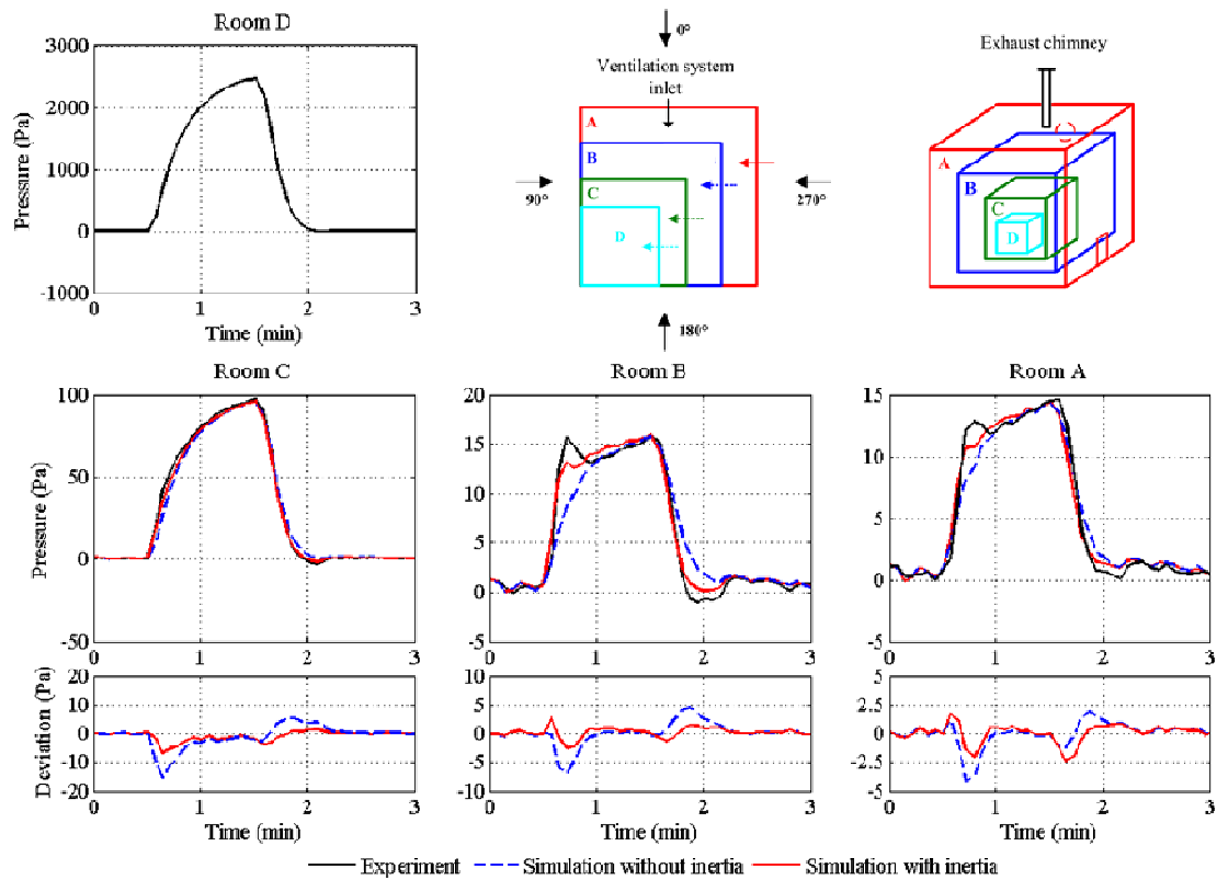
Figure 15: Experimental and numerical comparisons of internal room pressures (internal overpressure inside room D, without wind, ventilation system off).
