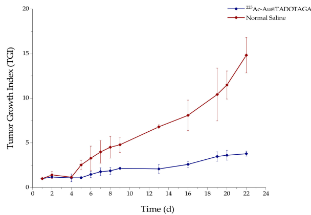
Figure 5. Effect of intratumoral injection of [ ^{225}\text{Ac} ] ^{225}\text{Ac-Au@TADOTAGA} (blue line) or normal saline (red line) on the tumor growth index (TGI) of U-87 MG tumor-bearing SCID mice. Values represent the mean \pm SD ( n = 5 mice per group).
