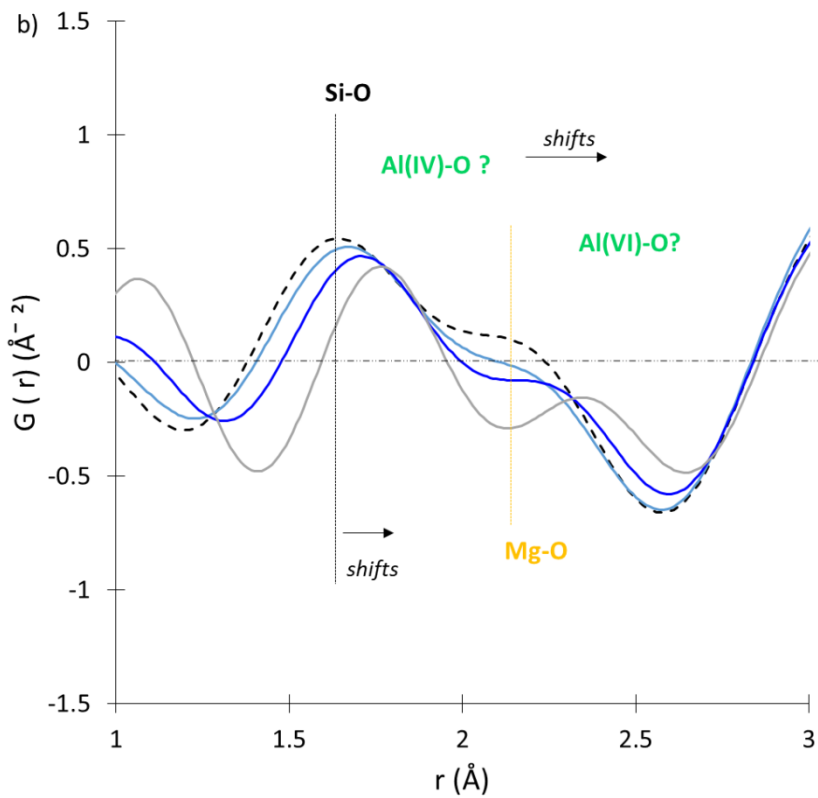
Figure 7: Reduced pair distribution function of M-A-S-H samples ( \text{Al/Si} = 0.05, 0.10, 0.15, 1 \text{ year} - 50^\circ\text{C} ) compared to M-S-H sample ( \text{Al/Si} = 0 ).
