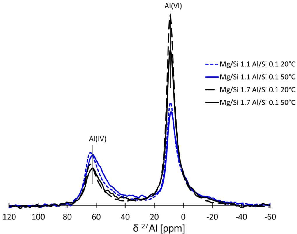
Figure S3: ^{27}\text{Al} MAS NMR spectra of M-A-S-H phases Mg/Si=1.1 and 1.7 at constant Al/Si=0.10: comparison between the samples cured during 1 year at 50°C and the samples cured during 2 years at 20°C.
