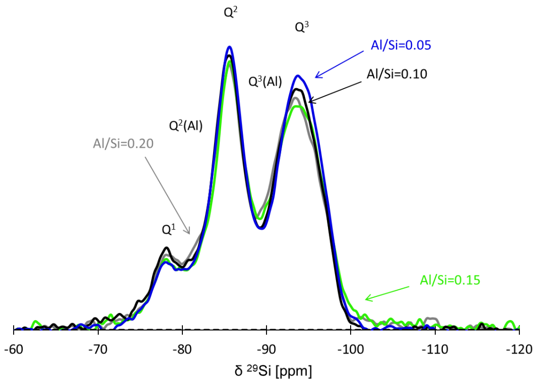
Figure S4: ^{29}\text{Si} MAS NMR spectra with assignments of Q^n environments of the M-A-S-H samples, Mg/Si=1.7 and Al/Si=0.05-0.20 (all samples cured for 1 year at 50°C).
