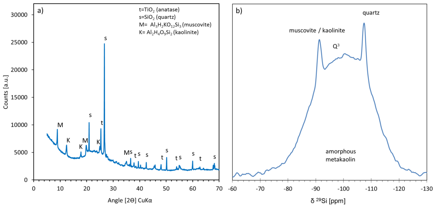
Figure 2 : a) XRD pattern and b) ^{29}\text{Si} MAS NMR spectrum of metakaolin ARGICAL-M 1200S.
