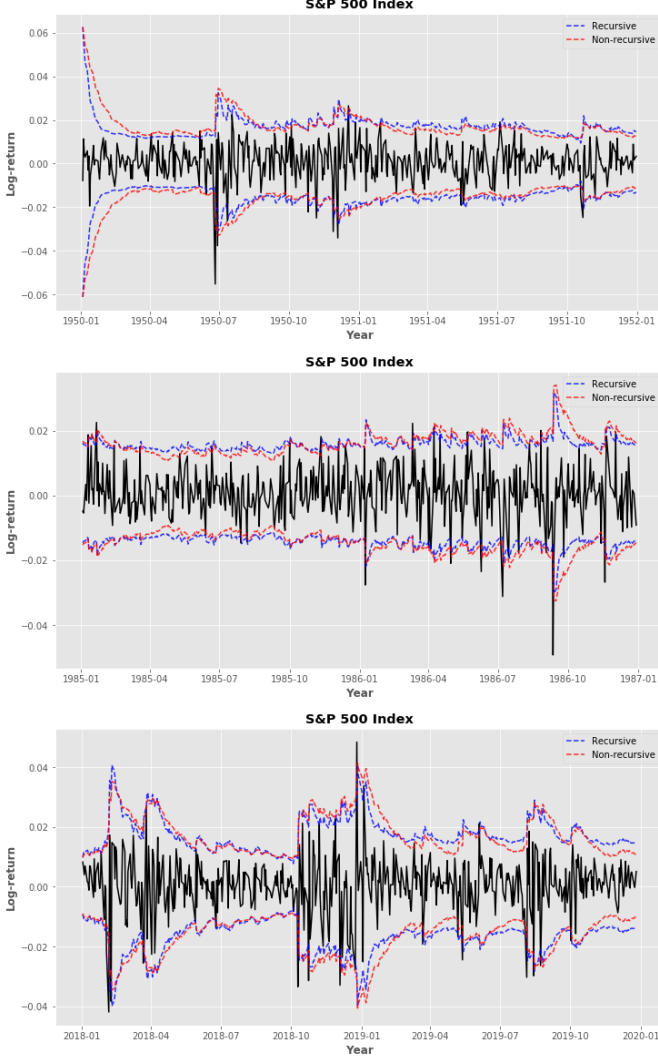
Figure 12: Log-returns r_t of S&P500 Index (solid lines) and confidence intervals \bar{r} \pm 1.96\hat{\sigma}_t and \bar{r} \pm 1.96\tilde{\sigma}_t (dotted lines) using the recursive \hat{\sigma}_t (blue) and non-recursive \tilde{\sigma}_t (red) predicted volatilities, respectively, where \bar{r} is the mean of the log-returns r_t . From top to bottom we have the periods: year 1950 to 1952, 1985 to 1987 and 2018 to 2020.
