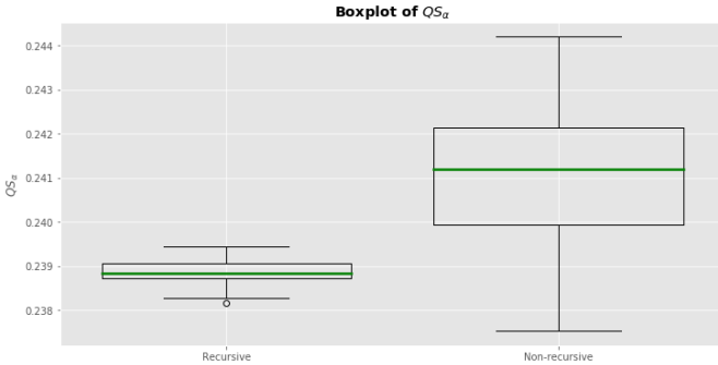
Figure 13: Boxplots of one hundred QS_\alpha scores with use of the recursive \hat{\sigma}_t and non-recursive \tilde{\sigma}_t volatility process, respectively, for \alpha = \{0.01, 0.02, \dots, 0.99\} , using the GARCH(1, 1) model on the log-returns r_t of S&P500 Index with random initial value in \mathcal{K} .
