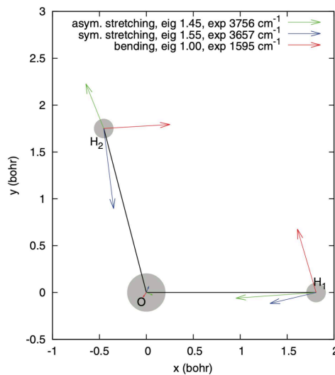
FIG. 8. Eigenvectors of the 3 \times 3 correlation matrix of QMC forces \mathbf{S}^{\text{QMC}} in the water monomer. The obtained eigenvectors correspond to the well-known three vibrational modes: bending (red), symmetrical (blue), and asymmetrical (green) stretching. The smaller eigenvalue corresponds to the lowest-frequency vibrational mode. The eigenvalues in the plot are all rescaled by the lowest one. Reprinted with permission from Luo et al. 110 , J. Chem. Phys. , published by AIP in 2014.
