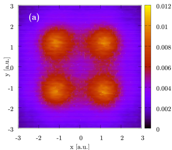
FIG. 10. The xy -plane charge density of the square four hydrogen ( H_4 ), calculated using a JAGP WF. Reprinted with permission from Genovese et al. 123 , J. Chem. Phys. , published by AIP in 2019.
