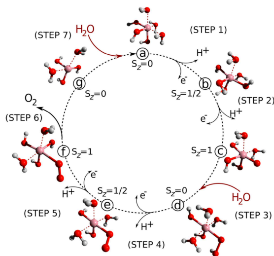
FIG. 19. Reaction cycle involving the cobalt ion model, studied in Ref. 175 by VMC and LRDMC. The pink, red, and white balls represent the cobalt, oxygen, and hydrogen atoms, respectively. Reprinted with permission from Chu et al. 175 , J. Chem. Theory Comput. , published by ACS in 2016.
