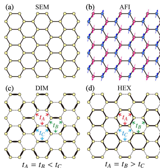
FIG. 17. The graphene structures studied in Ref. 165. (a) SEM honeycomb, semimetallic; (b) AFI honeycomb antiferromagnetic insulator; (c) DIM dimerized Kekulé-like insulator; (d) HEX distorted hexagonal insulator. There are two carbons per unit cell in (a) and (b), six in (c) and (d). t_A , t_B , and t_C schematically denote different hopping integrals magnitudes. Reprinted with permission from Sorella et al. 165 , Phys. Rev. Lett. , published by APS in 2018.
