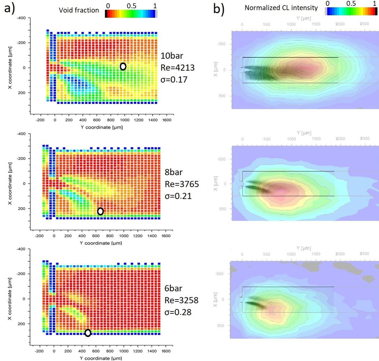
Figure 3 - a) The overlap of the void fraction mapping and the maximum CL activity position (black circle) of the 2d gaussian data fit for MD-A. b) shadowgraphy average image (black indicating high void fraction regions) of the flow in microchannels (average cloud cover) overlapped with the contour maps of the CL activity in MD-A. The bubble collapse region, indicated by the maximum CL activity, is observed at the end of the main cavitation cloud. Flow is from left to right.
