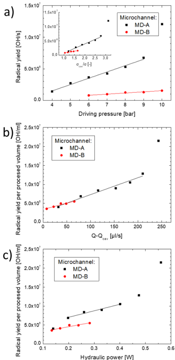
Figure 6 - Radical production figures for the MD-A (black) and -B (red). a) Radical yield at different driving pressures and \sigma_{cav}/\sigma parameter values (in subplot), b) Radical yield per processed volume as a function of the Q-Q_{cav} parameter (volume flow above cavitation inception flow), c) Radical yield per processed volume at different hydraulic power.
