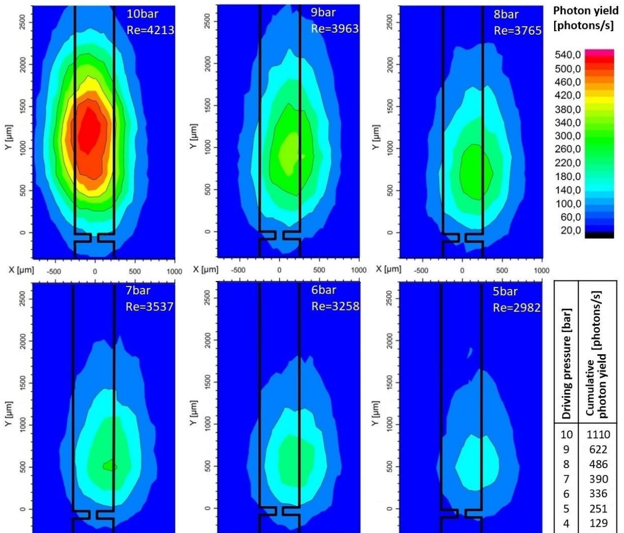
Figure 2 – The contour plot of the chemiluminescence intensity in the MD-A as a function of \Delta P (4 bar plot omitted for clarity). Flow direction is from bottom to top, with the black lines represent the channel walls. The measurement points were acquired every 100 \mu m in the x and 200 \mu m in the y coordinate, and the photon yield averaged over 3s. The cumulative CL yield with subtracted background signal values for each driving pressure is tabled in the lower right corner.
