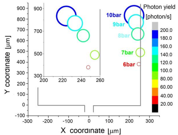
Figure 5 - The intensity and position of the maximum CL activity downstream the constriction as a function of increasing pressure in MD-B. A rudimentary 2D gaussian plot of the acquired data points was performed to approximate the highest intensity and position of the CL emission axis. Flow is the y-axis.
