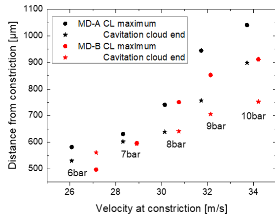
Figure 4 - MD-A and MD-B channel: the distance of the maximum CL activity (circle), the cavitation cloud end (star) from the diaphragm opening at different jet velocities emerging from the constriction (driving pressures indicated).
